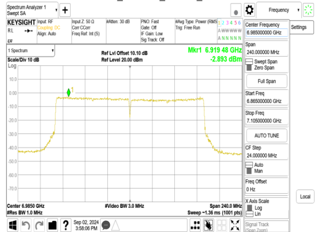
802.11be_160MHz_Chain0_6985MHz_996+484+242_MRU2
