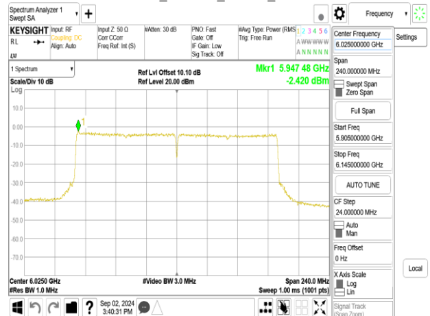
802.11be_160MHz_Chain0_6025MHz_996+484+242_MR2
