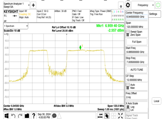
802.11be_80MHz_Chain1_6945MHz_484+242_MRU2
