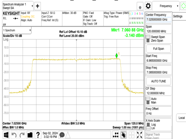
802.11be_80MHz_Chain0_7025MHz_484+242_MRU1
