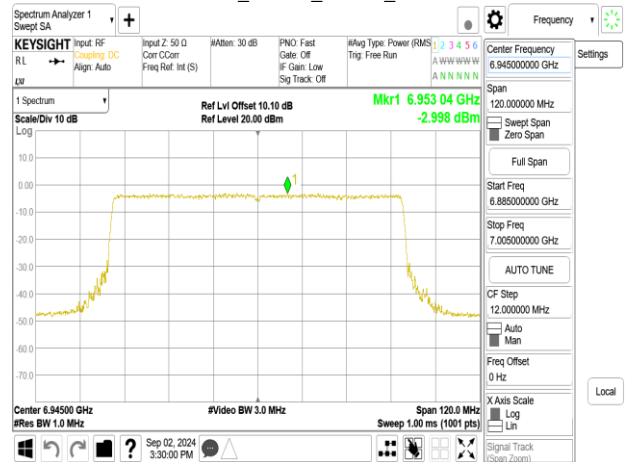
802.11be_80MHz_Chain0_6945MHz_484+242_MR2
