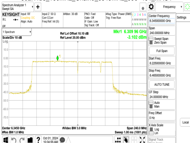
802.11be_160MHz_Chain0_6345MHz_996+484_MR1
