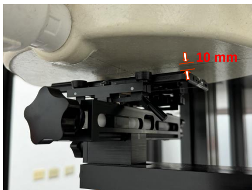
Photograph 11. Hotspot, Back Surface, 10mm
