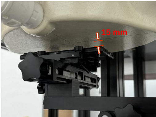
Photograph 23. Body-worn, Back Surface, 15mm
