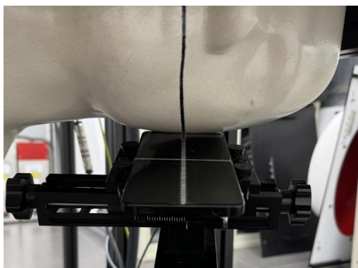
Photograph 7. Head, Left Tilt, 0mm
