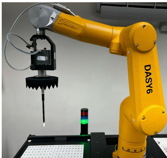
Fig.2 Photograph of the mmW measurement system
