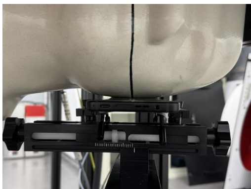
Photograph 5. Head, Left Touch, 0mm
