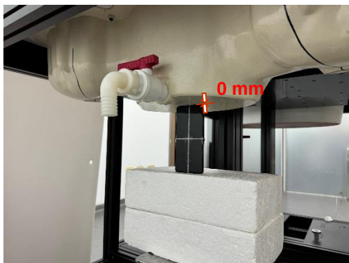
Photograph 29. Extremity, Top Edge, 0mm
