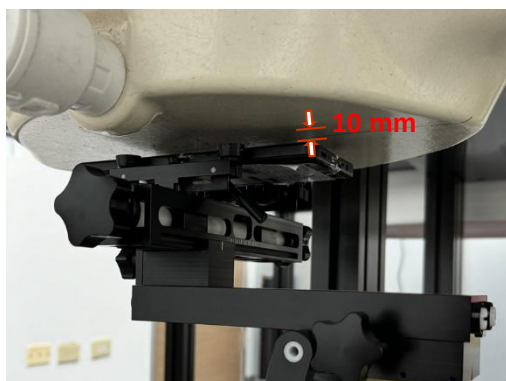
Photograph 9. Hotspot, Front Surface, 10mm
