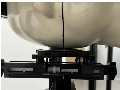
Photograph 1. Head, Right Touch, 0mm
