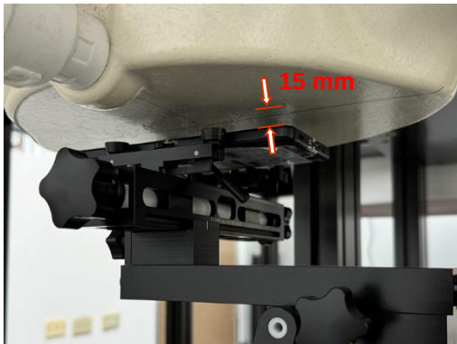
Photograph 21. Body-worn, Front Surface, 15mm
