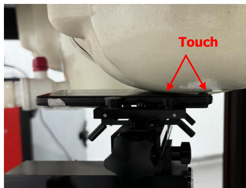
Photograph 6. Head, Left Touch, 0mm
