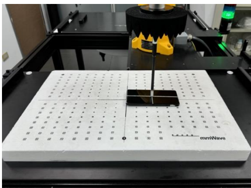
Photograph 37. PD, Front Surface, 2mm
