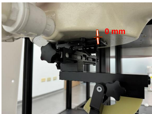
Photograph 27. Extremity, Back Surface, 0mm
