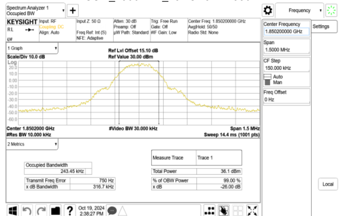
GSM_1900MHz_LowCH512-1850.2
