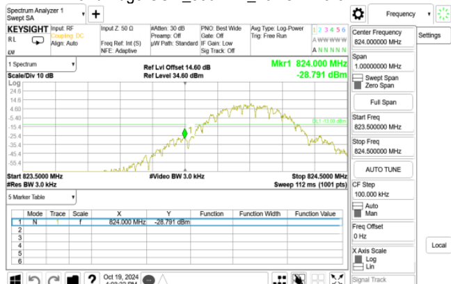
Band Edge GSM_850MHz_LowCH128-824.2
