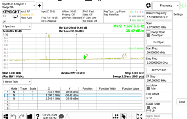
EDGE_850MHz_HighCH251-848.8
