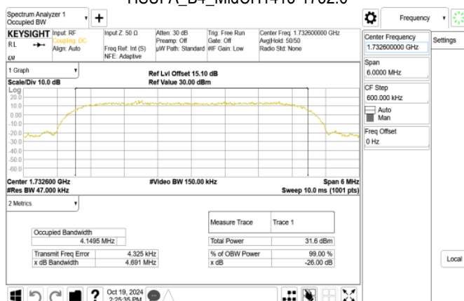
HSUPA_B4_MidCH1413-1732.6
