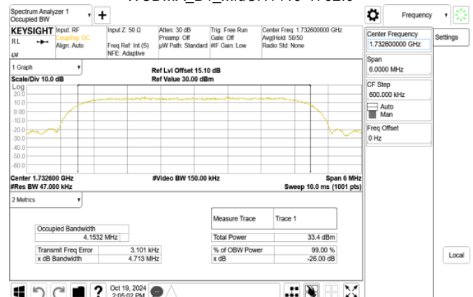
WCDMA_B4_MidCH1413-1732.6
