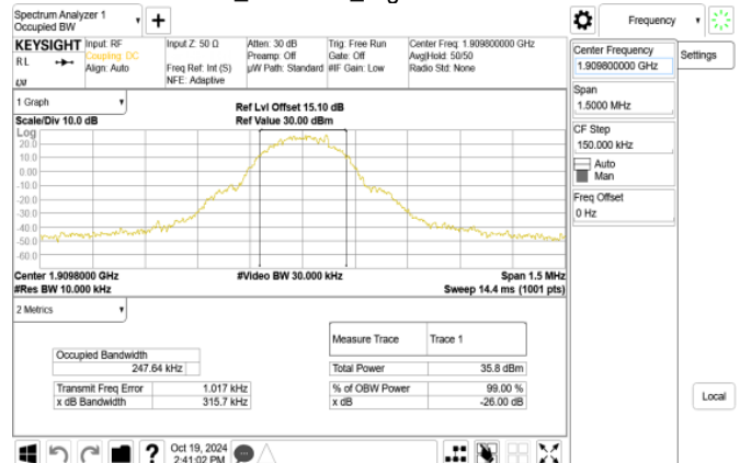
GSM_1900MHz_HighCH810-1909.8
