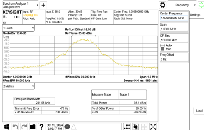
GPRS_1900MHz_HighCH810-1909.8
