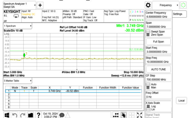
GSM_850MHz_MidCH190-836.6
