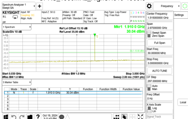
GPRS_1900MHz_HighCH810-1909.8
