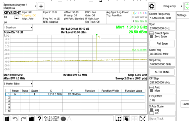
EDGE_1900MHz_HighCH810-1909.8
