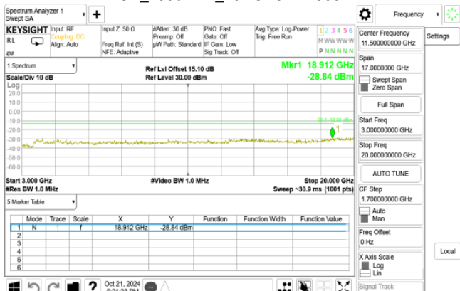
EDGE_1900MHz_LowCH512-1850.2
