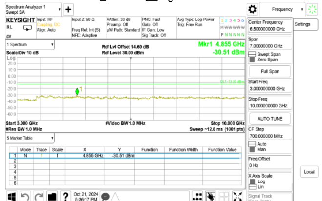
EDGE_850MHz_HighCH251-848.8
