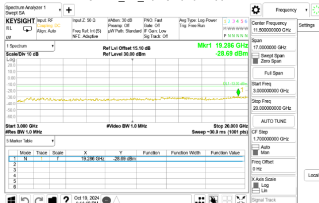
WCDMA_B2_LowCH9262-1852.4
