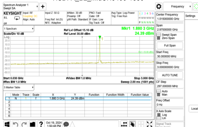
HSDPA_B2_MidCH9400-1880
