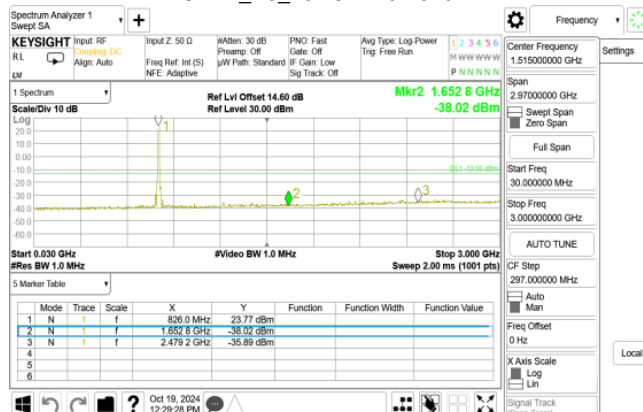
HSDPA_B5_MidCH4183-836.6
