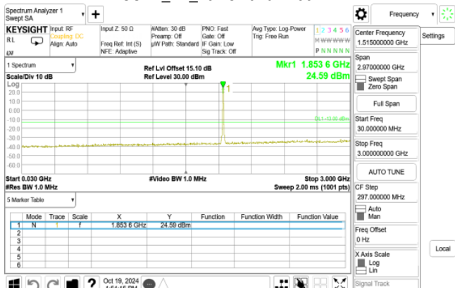
HSUPA_B2_LowCH9262-1852.4
