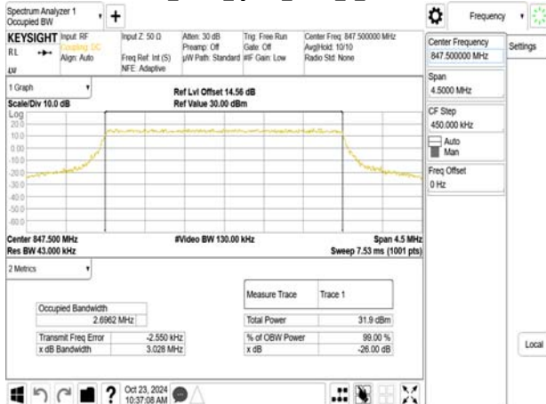
Band5_3MHz_QPSK_RB15_0_CH20635
