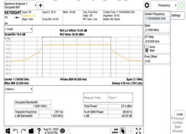
Band4_1.4MHz_256QAM_RB6_0_CH20393
