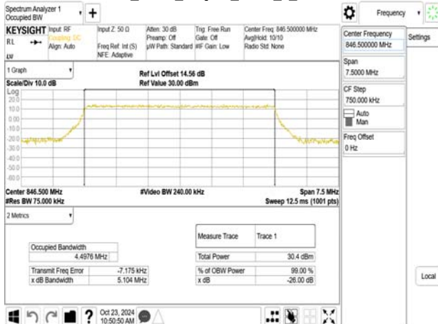
Band5_5MHz_64QAM_RB25_0_CH20625
