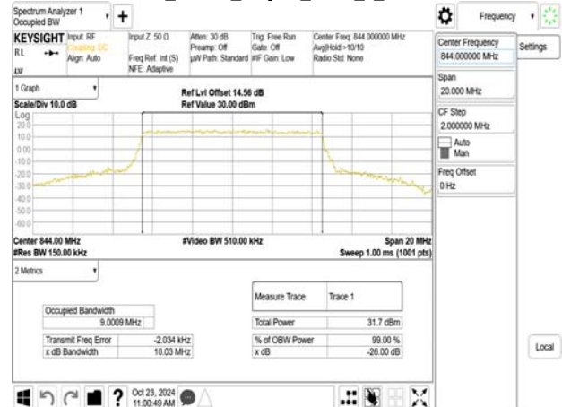
Band5_10MHz_16QAM_RB50_0_CH20600
