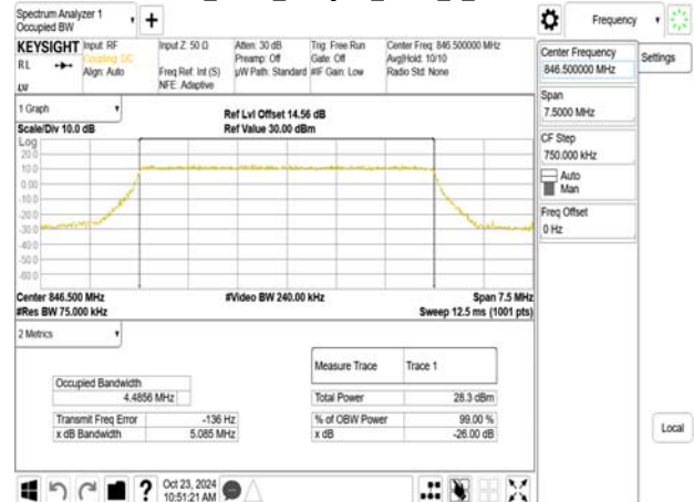
Band5_5MHz_256QAM_RB25_0_CH20625
