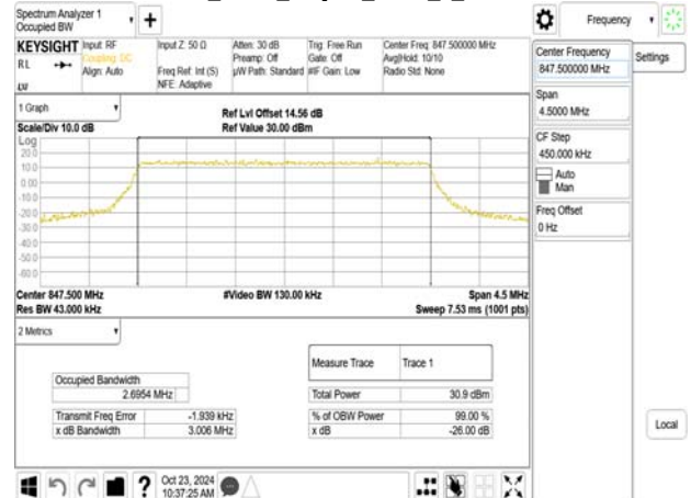
Band5_3MHz_16QAM_RB15_0_CH20635
