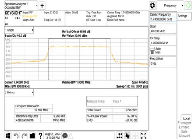
Band4_20MHz_256QAM_RB100_0_CH20300
