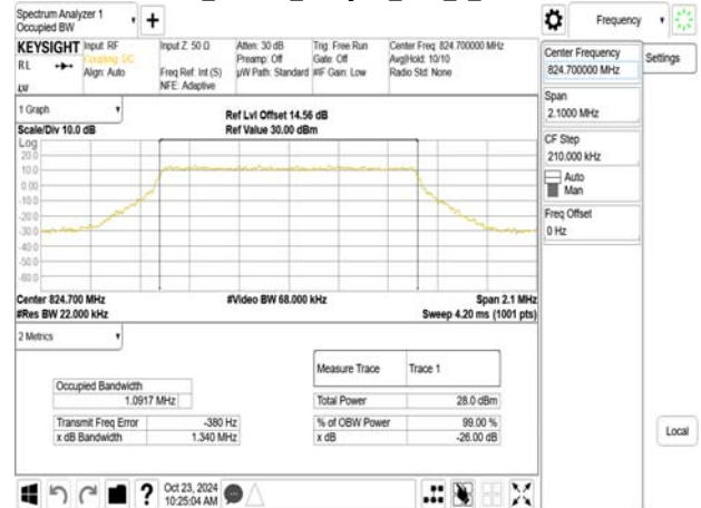
Band5_1.4MHz_256QAM_RB6_0_CH20525
