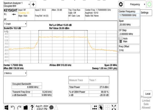
Band4_10MHz_256QAM_RB50_0_CH20350
