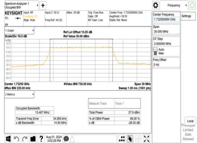
Band4_15MHz_256QAM_RB75_0_CH20325
