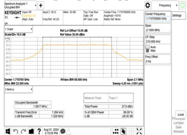
Band4_1.4MHz_256QAM_RB6_0_CH20175
