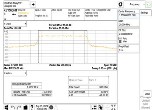
Band4_10MHz_16QAM_RB50_0_CH20350
