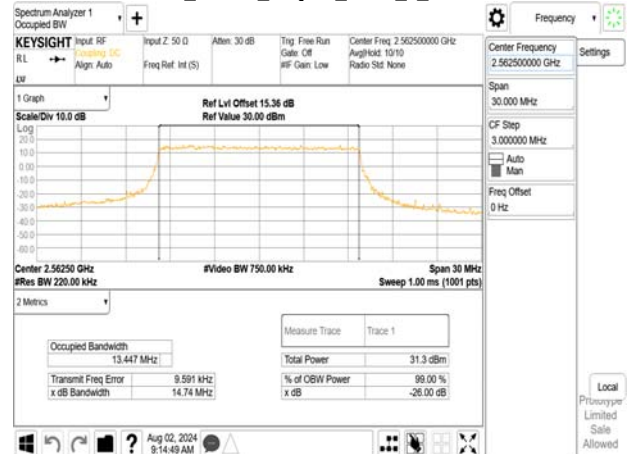
Band7_15MHz_16QAM_RB75_0_CH21375
