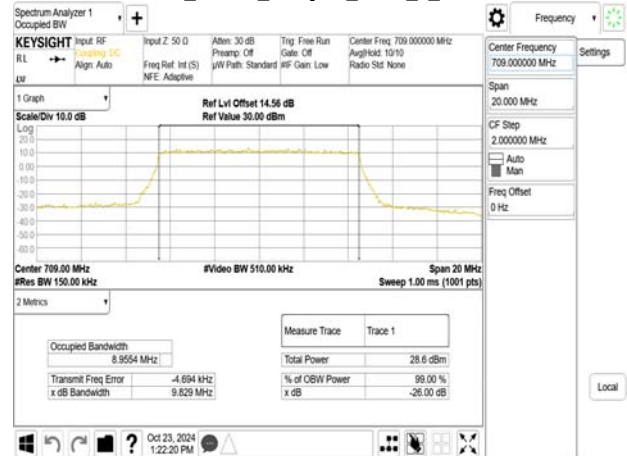
Band17_10MHz_256QAM_RB50_0_CH23790
