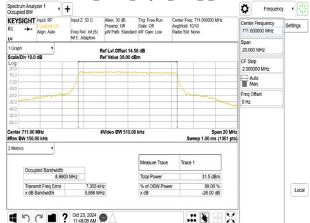
Band12_10MHz_16QAM_RB50_0_CH23130
