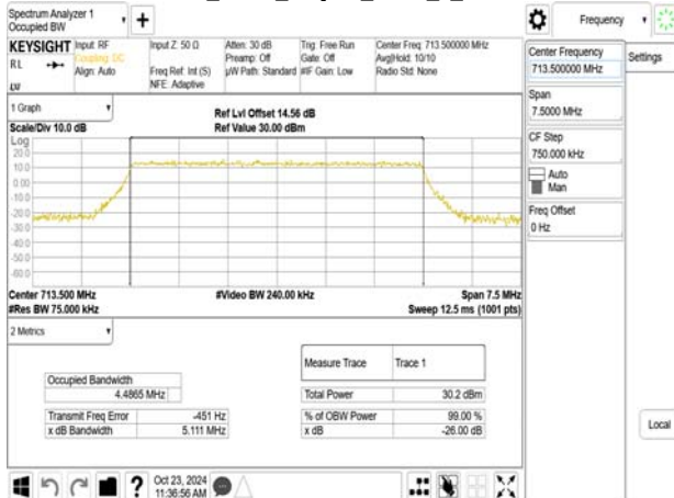
Band12_5MHz_64QAM_RB25_0_CH23155
