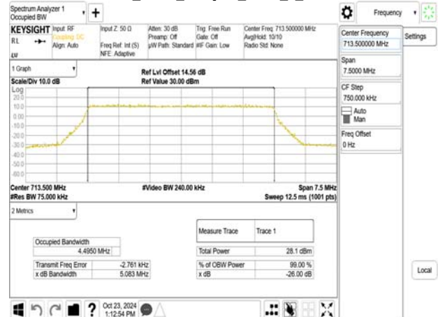
Band17_5MHz_256QAM_RB25_0_CH23825
