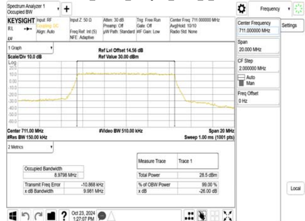
Band17_10MHz_256QAM_RB50_0_CH23800
