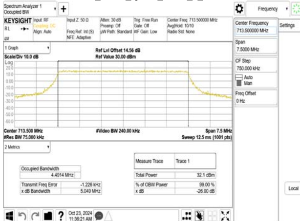
Band12_5MHz_QPSK_RB25_0_CH23155
