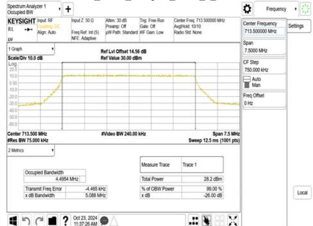
Band12_5MHz_256QAM_RB25_0_CH23155
