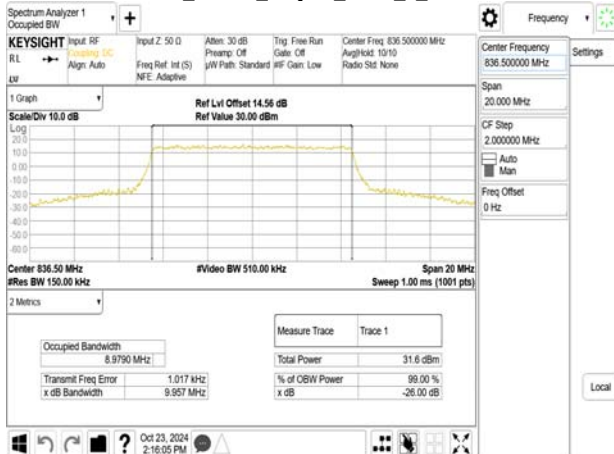
Band26_10MHz_16QAM_RB50_0_CH26915
