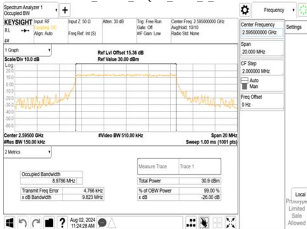
Band38_10MHz_16QAM_RB50_0_CH38200
