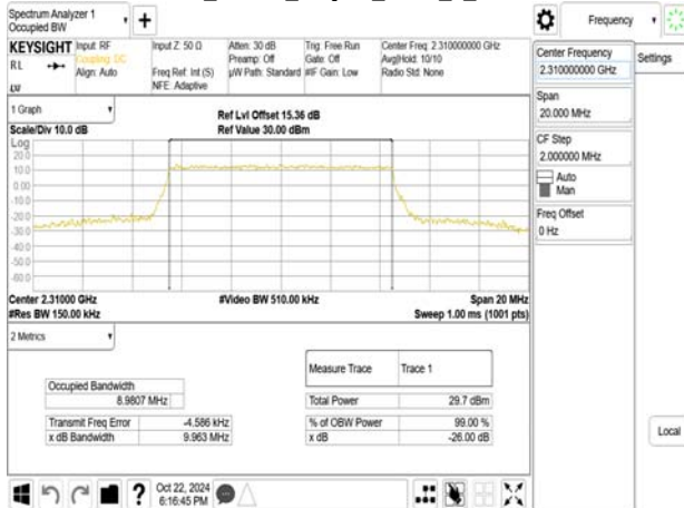
Band30_10MHz_256QAM_RB50_0_CH27710
