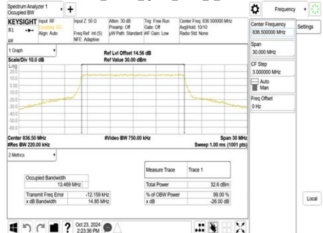
Band26_15MHz_QPSK_RB75_0_CH26915
