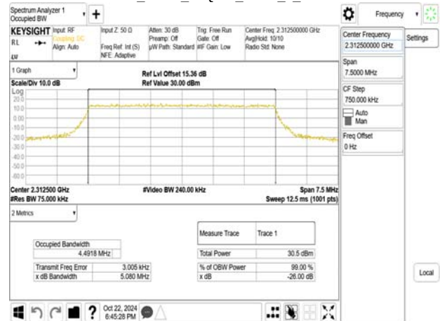
Band30_5MHz_64QAM_RB25_0_CH27685
