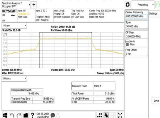
Band26_15MHz_16QAM_RB75_0_CH26915
