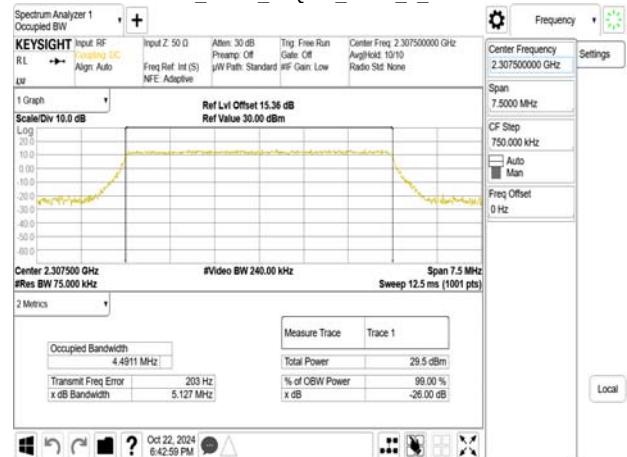
Band30_5MHz_64QAM_RB25_0_CH27710
