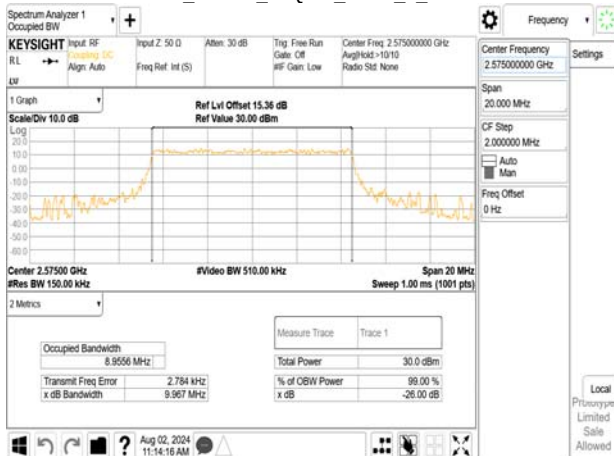
Band38_10MHz_64QAM_RB50_0_CH37800
