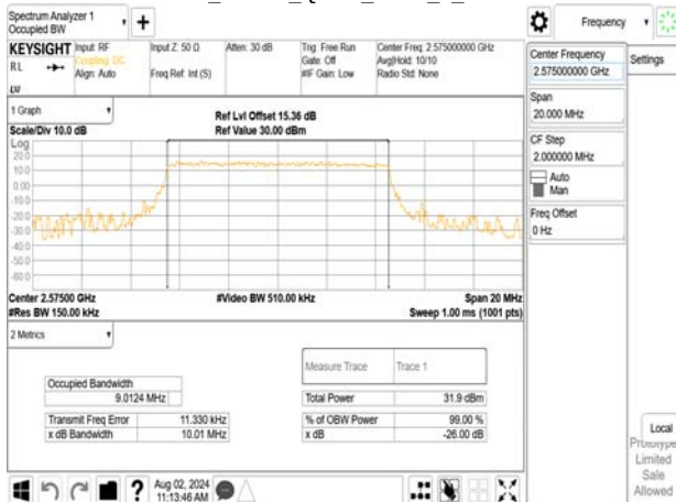
Band38_10MHz_QPSK_RB50_0_CH37800
