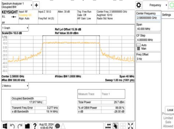
Band38_20MHz_64QAM_RB100_0_CH37850
