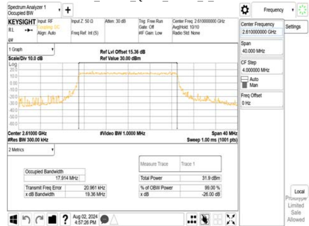
Band38_20MHz_16QAM_RB100_0_CH37850
