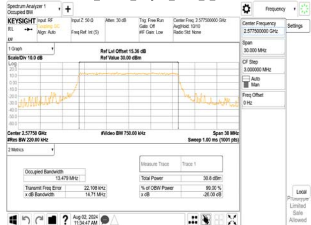
Band38_15MHz_16QAM_RB75_0_CH37825
