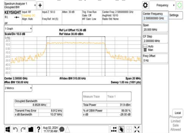
Band38_10MHz_QPSK_RB50_0_CH38200
