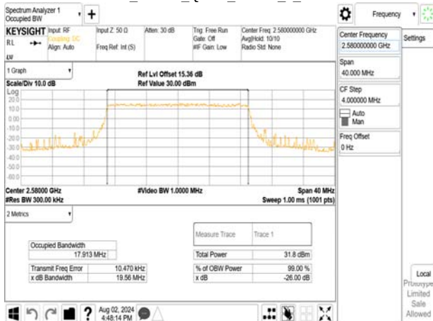
Band38_20MHz_QPSK_RB100_0_CH37850
