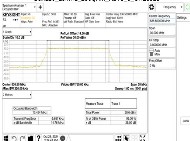
Band26_15MHz_256QAM_RB75_0_CH26915
