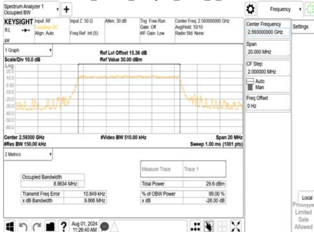
Band41_10MHz_256QAM_RB50_0_CH40620
