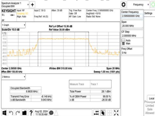
Band38_10MHz_256QAM_RB50_0_CH38200
