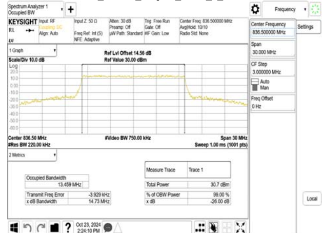
Band26_15MHz_64QAM_RB75_0_CH26915
