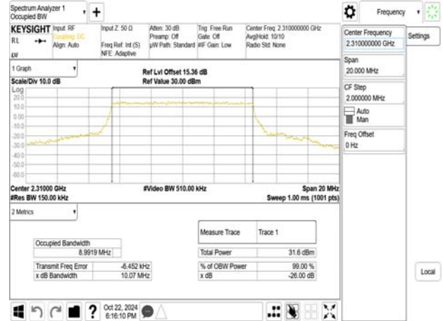
Band30_10MHz_16QAM_RB50_0_CH27710
