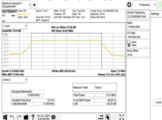
Band30_5MHz_256QAM_RB25_0_CH27710
