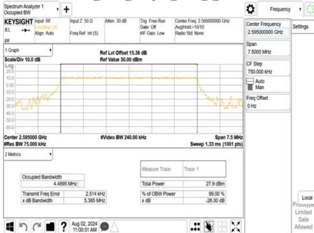
Band38_5MHz_256QAM_RB25_0_CH38225
