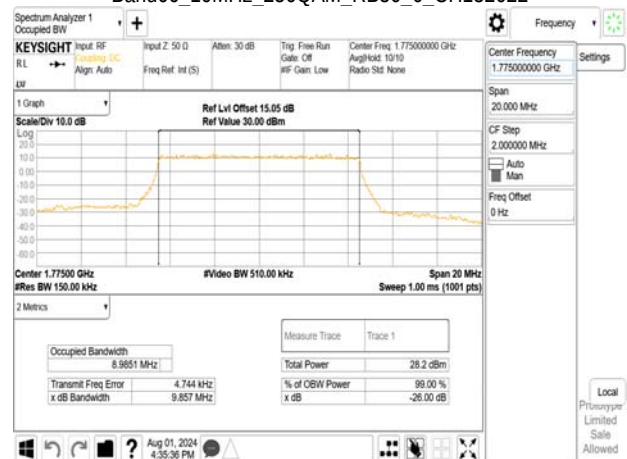
Band66_10MHz_256QAM_RB50_0_CH132622
