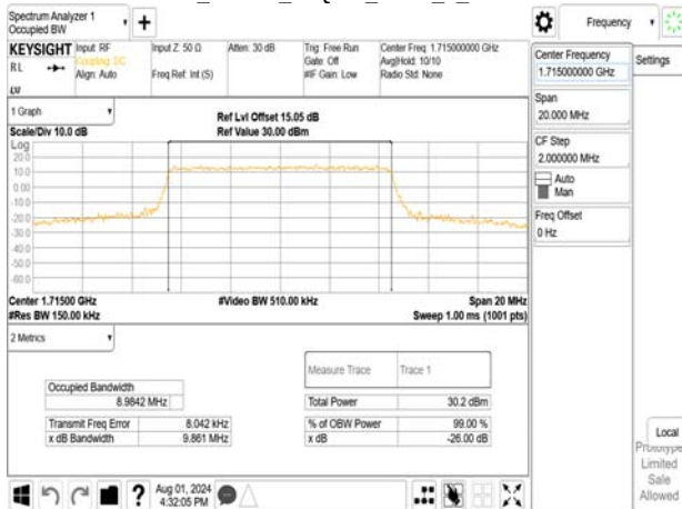
Band66_10MHz_64QAM_RB50_0_CH13222
