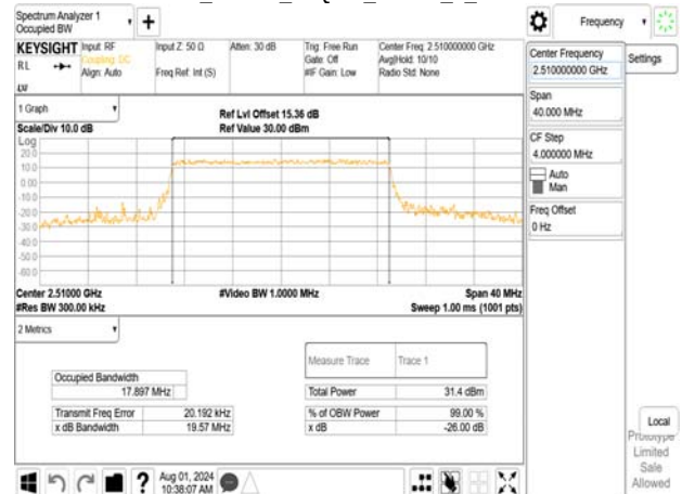
Band41_20MHz_64QAM_RB100_0_CH39790
