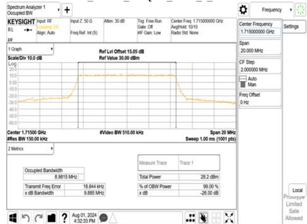
Band66_10MHz_256QAM_RB50_0_CH13222
