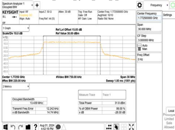
Band66_15MHz_QPSK_RB75_0_CH132597
