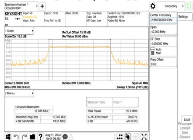
Band41_20MHz_256QAM_RB100_0_CH41490
