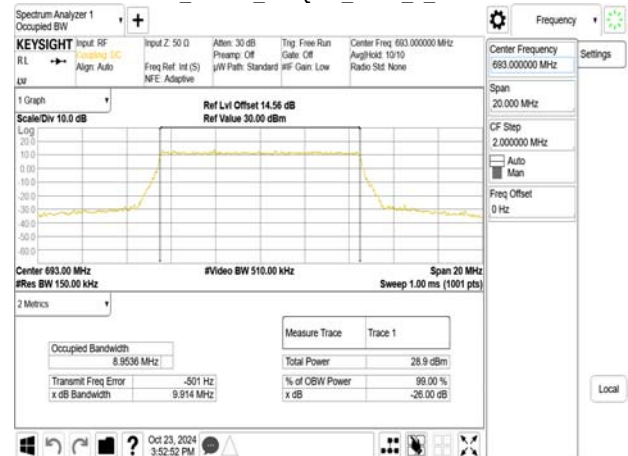
Band71_10MHz_256QAM_RB50_0_CH133422
