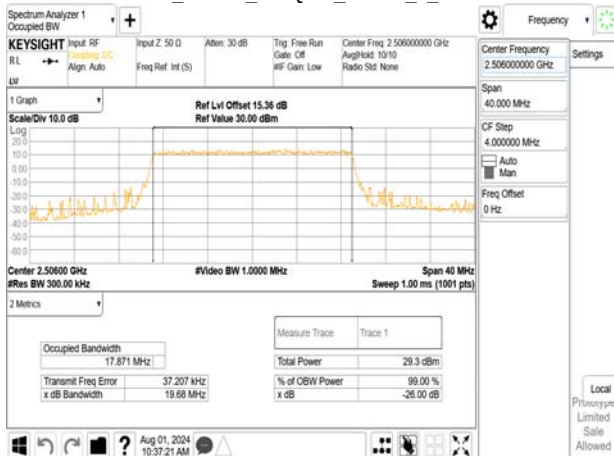
Band41_20MHz_256QAM_RB100_0_CH39750
