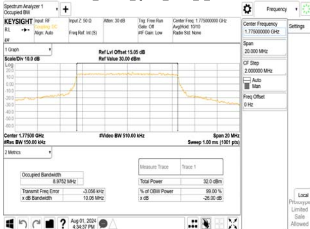
Band66_10MHz_QPSK_RB50_0_CH132622
