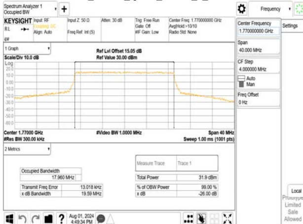
Band66_20MHz_QPSK_RB100_0_CH132572
