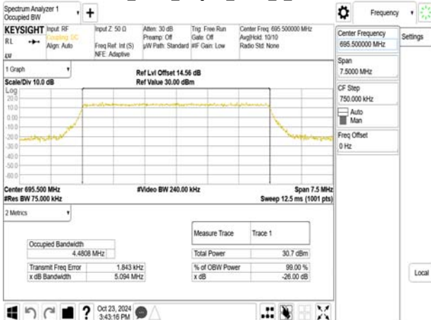
Band71_5MHz_64QAM_RB25_0_CH133447
