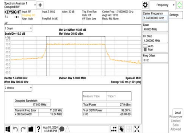
Band66_20MHz_256QAM_RB100_0_CH132572
