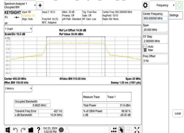
Band71_10MHz_16QAM_RB50_0_CH133422
