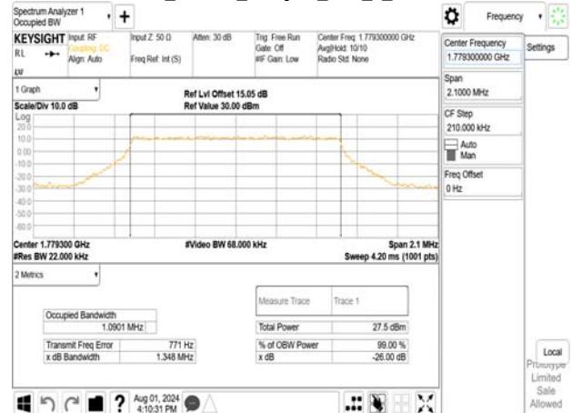
Band66_1.4MHz_256QAM_RB6_0_CH132665
