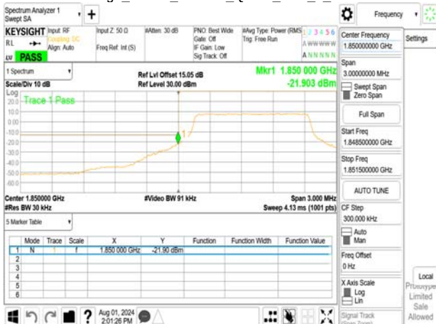
Band Edge_Band2_1.4MHz_QPSK_RB6_0_CH18607
