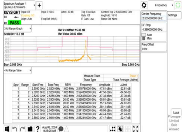
Emission Mask_Band7_10MHz_QPSK_RB1_49_CH21100
