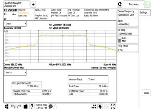
Band71_20MHz_16QAM_RB100_0_CH133372
