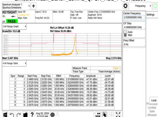
Emission Mask_Band7_15MHz_QPSK_RB1_74_CH21100
