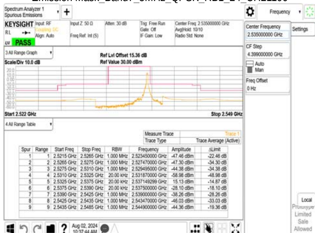
Emission Mask_Band7_5MHz_QPSK_RB1_24_CH21100
