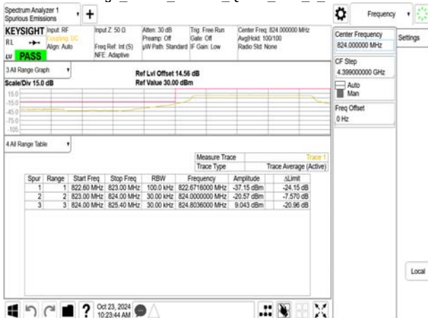
Band Edge_Band5_1.4MHz_QPSK_RB6_0_CH20407
