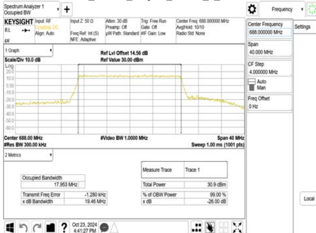
Band71_20MHz_64QAM_RB100_0_CH133372
