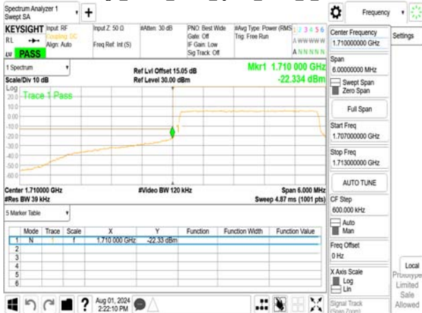
Band Edge_Band4_3MHz_QPSK_RB15_0_CH20385
