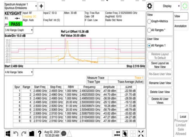
Emission Mask_Band7_5MHz_QPSK_RB1_0_CH21100
