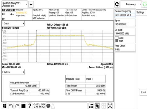
Band71_15MHz_64QAM_RB75_0_CH133397
