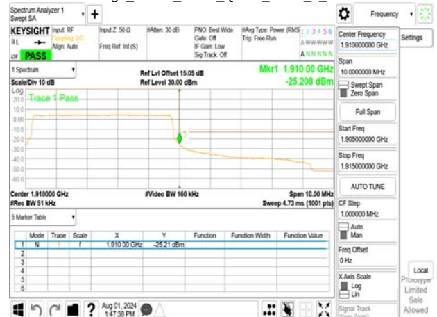
Band Edge_Band2_5MHz_QPSK_RB25_0_CH19175
