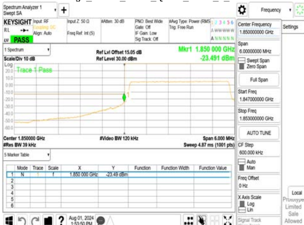
Band Edge_Band2_3MHz_QPSK_RB15_0_CH18185
