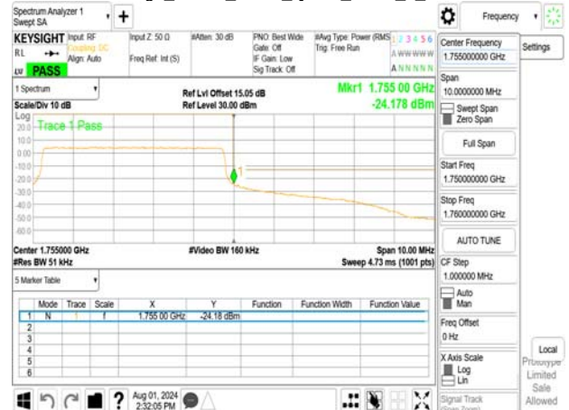
Band Edge_Band4_5MHz_QPSK_RB25_0_CH20375
