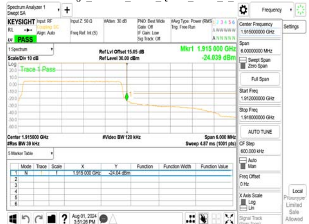
Band Edge_Band25_3MHz_QPSK_RB15_0_CH26675
