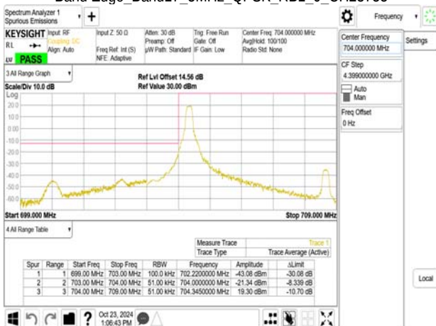
Band Edge_Band17_5MHz_QPSK_RB1_0_CH23755
