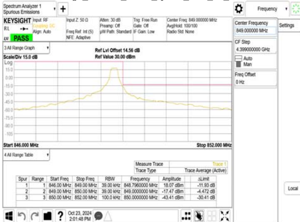
Band Edge_Band26_3MHz_QPSK_RB15_0_CH26805
