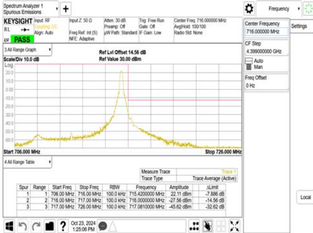
Band Edge_Band17_10MHz_QPSK_RB50_0_CH23780
