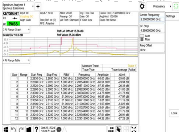
Emission Mask_Band30_5MHz_QPSK_RB1_24_CH27710
