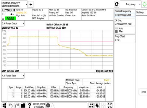
Band Edge_Band26_15MHz_QPSK_RB75_0_CH26965
