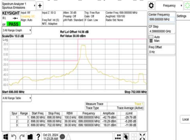
Band Edge_Band12_3MHz_QPSK_RB1_0_CH23025
