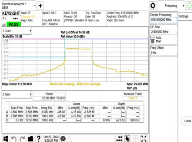
Emission Mask_Band26-Part90s_5MHz_QPSK_RB25_0_CH26715
