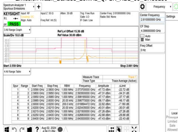
Emission Mask_Band38_20MHz_QPSK_RB1_99_CH38150
