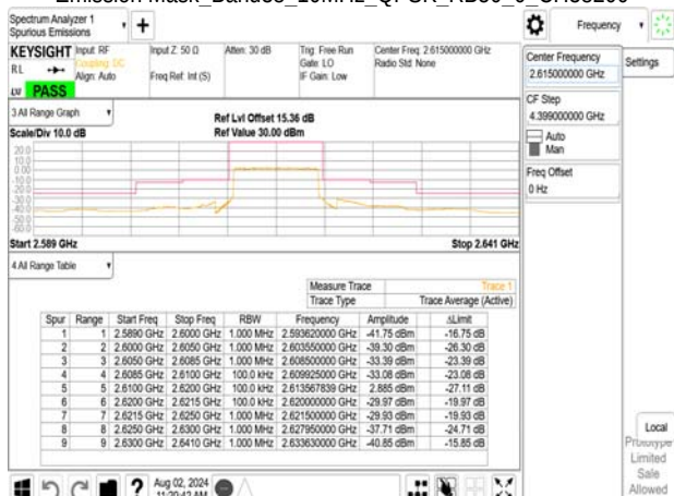
Emission Mask_Band38_10MHz_QPSK_RB50_0_CH38200
