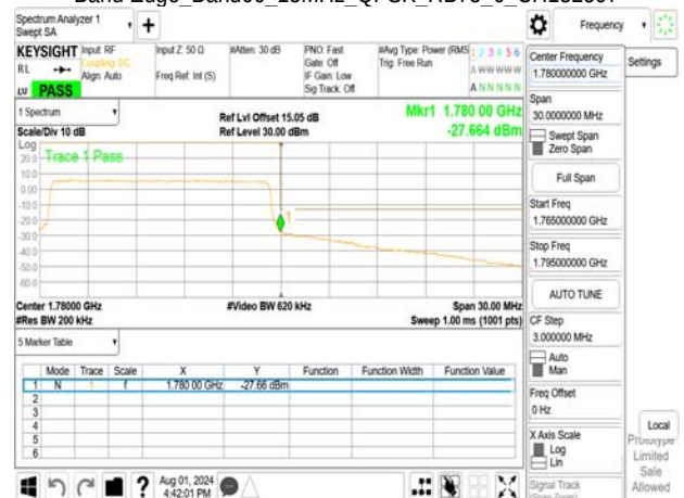
Band Edge_Band66_15MHz_QPSK_RB75_0_CH132597
