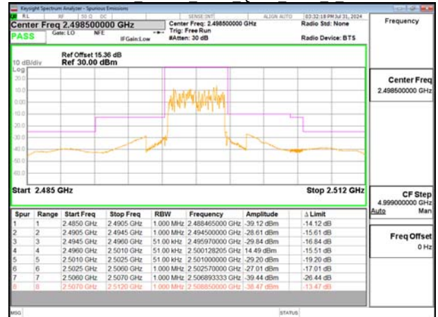
Emission Mask Band41 5MHz QPSK RB25 0 CH39675
