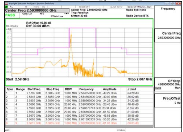
Emission Mask Band41_5MHz_QPSK_RB1_0_CH40620
