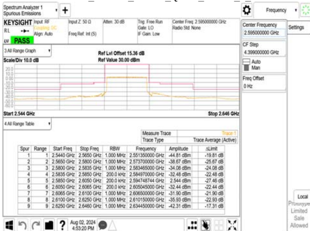
Emission Mask Band38_20MHz_QPSK_RB100_0_CH38150
