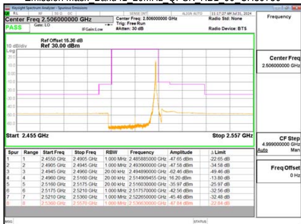
Emission Mask Band41 20MHz QPSK RB1 99 CH39750
