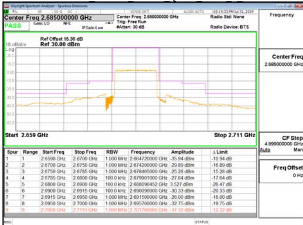
Emission Mask_Band41_10MHz_QPSK_RB50_0_CH41540
