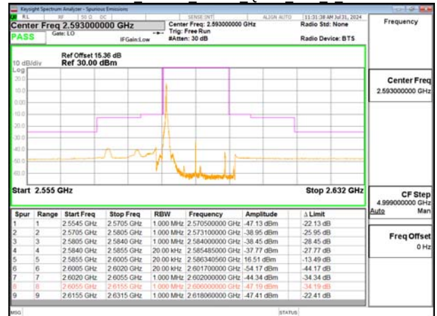
Emission Mask_Band41_15MHz_QPSK_RB1_0_CH40620
