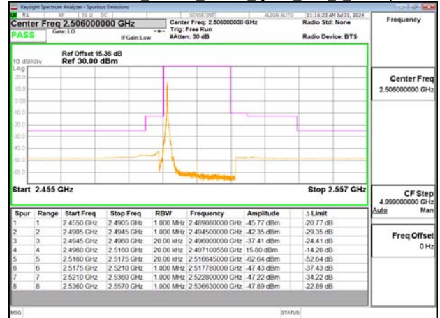
Emission Mask_Band41_20MHz_QPSK_RB1_0_CH39750
