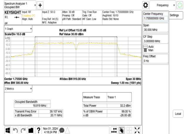
Band66B_10MHz+10MHz_16QAM_RB50-0+RB50-0_CH132373+CH132472
