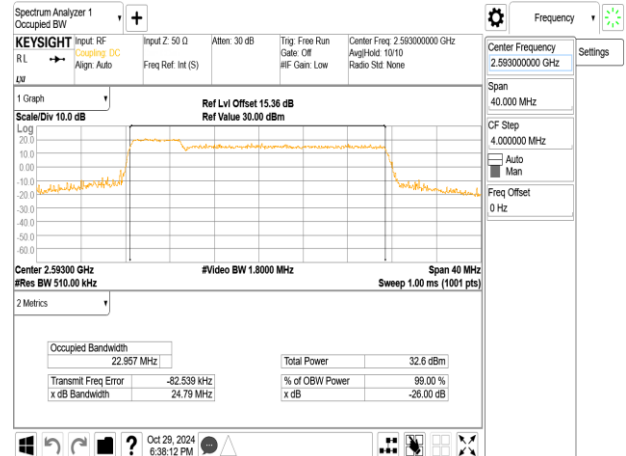
Band41_5MHz+20MHz_16QAM_RB25-0+RB100-0_CH40528+CH40645
