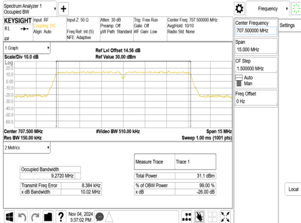
Band12B_5MHz+5MHz_256QAM_RB25-0+RB25-0_CH23071+CH23119
