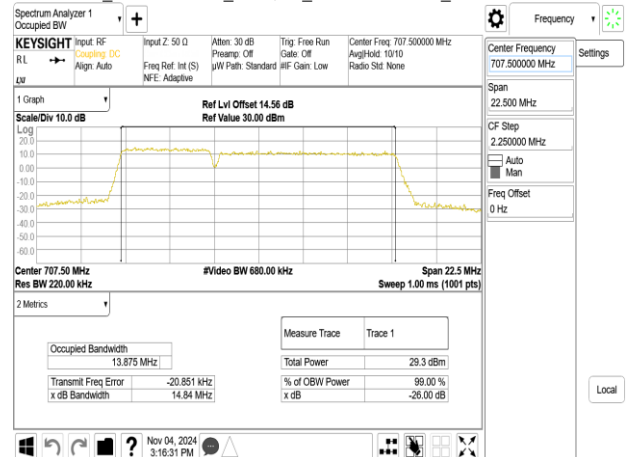
Band12B_5MHz+10MHz_256QAM_RB25-0+RB50-0_CH23048+CH23120
