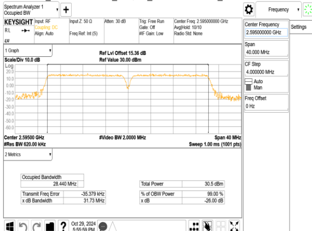
Band38_15MHz+15MHz_64QAM_RB75-0+RB75-0_CH37925+CH38075
