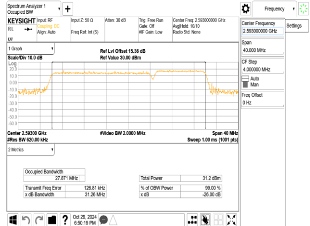
Band41_20MHz+10MHz_256QAM_RB100-0+RB50-0_CH40571+CH40715
