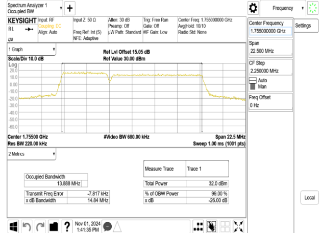
Band66B_5MHz+10MHz_16QAM_RB25-0+RB50-0_CH132375+CH132447
