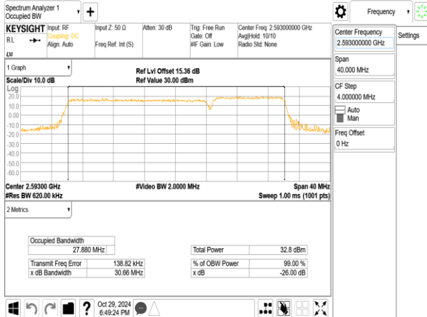
Band41_20MHz+10MHz_16QAM_RB100-0+RB50-0_CH40571+CH40715
