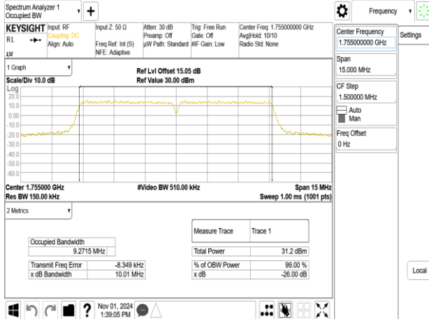
Band66B_5MHz+5MHz_64QAM_RB25-0+RB25-0_CH132398+CH132446
