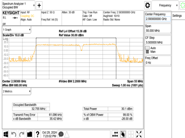
Band41_20MHz+20MHz_QPSK_RB100-0+RB100-0_CH40521+CH40719
