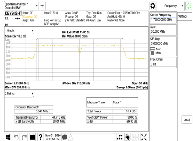
Band66B_10MHz+10MHz_64QAM_RB50-0+RB50-0_CH132373+CH132472
