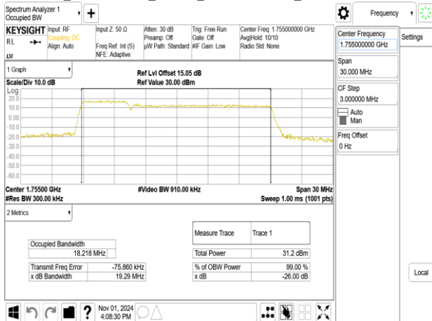
Band66B_5MHz+15MHz_256QAM_RB25-0+RB75-0_CH132353+CH132446
