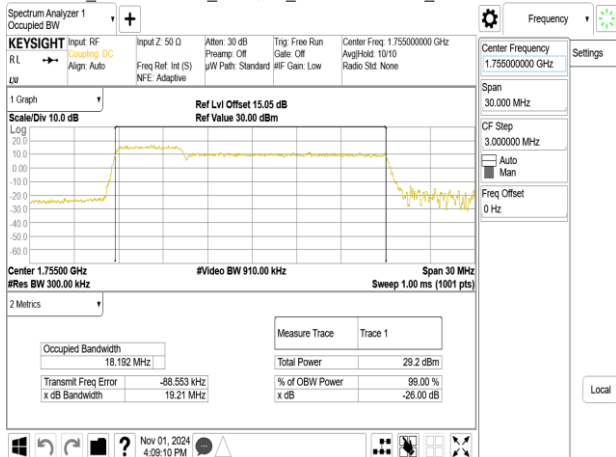
Band66B_5MHz+15MHz_256QAM_RB25-0+RB75-0_CH132353+CH132446
