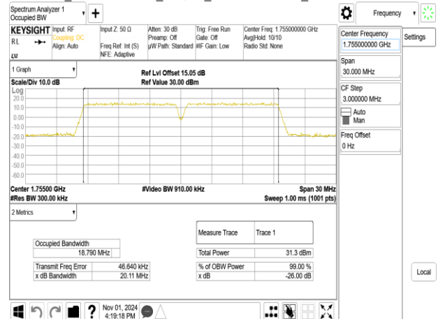
Band66B_10MHz+10MHz_64QAM_RB50-0+RB50-0_CH132373+CH132472
