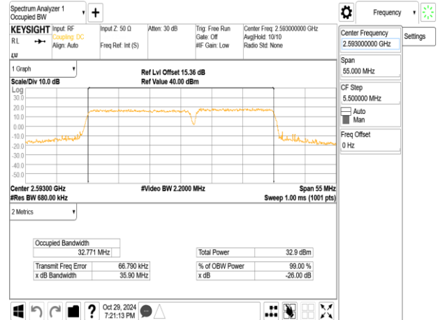
Band41_20MHz+15MHz_16QAM_RB100-0+RB75-0_CH40546+CH40717
