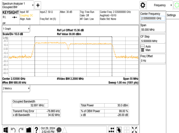
Band7_15MHz+20MHz_256QAM_RB75-0+RB100-0_CH21003+CH21174
