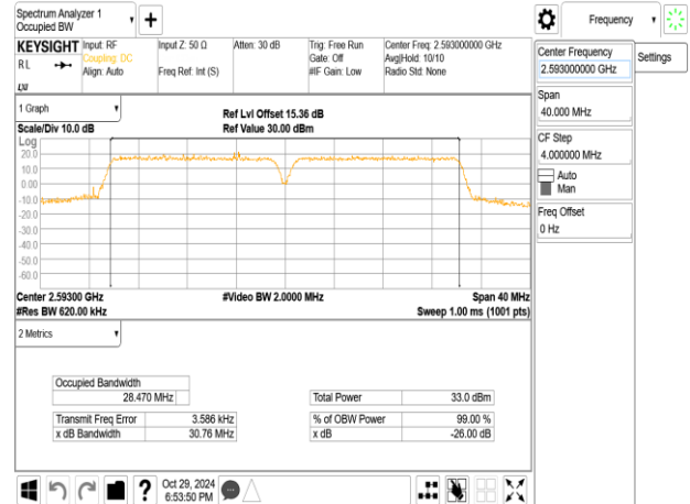
Band41_15MHz+15MHz_16QAM_RB75-0+RB75-0_CH40545+CH40695
