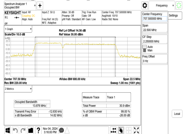
Band12B_5MHz+10MHz_256QAM_RB25-0+RB50-0_CH23048+CH23120
