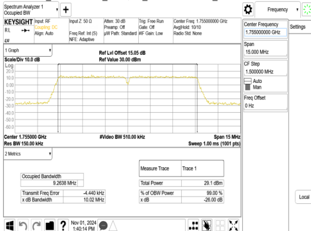
Band66B_5MHz+5MHz_256QAM_RB25-0+RB25-0_CH132398+CH132446
