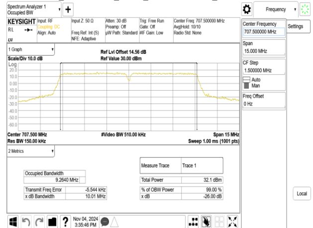
Band12B_5MHz+5MHz_16QAM_RB25-0+RB25-0_CH23071+CH23119
