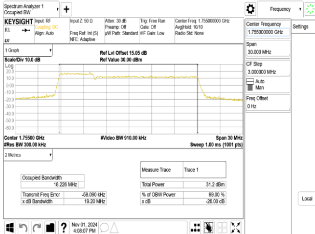
Band66B_5MHz+15MHz_64QAM_RB25-0+RB75-0_CH132353+CH132446
