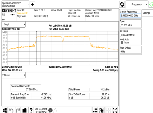
Band38_20MHz+20MHz_64QAM_RB100-0+RB100-0_CH37901+CH38099
