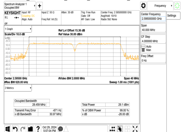
Band38_20MHz+20MHz_QPSK_RB100-0+RB100-0_CH37901+CH38099
