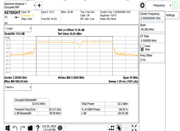
Band41_20MHz+15MHz_64QAM_RB100-0+RB75-0_CH40546+CH40717
