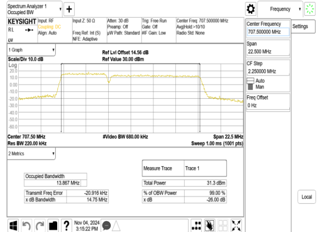
Band12B_5MHz+10MHz_64QAM_RB25-0+RB50-0_CH23048+CH23120
