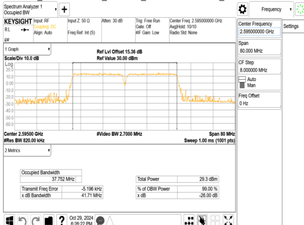
Band38_20MHz+20MHz_256QAM_RB100-0+RB100-0_CH37901+CH38099
