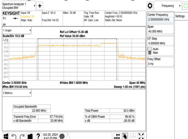
Band41_20MHz+5MHz_16QAM_RB100-0+RB25-0_CH40595+CH40712
