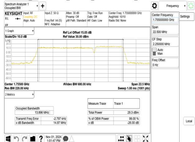
Band66B_5MHz+15MHz_QPSK_RB25-0+RB75-0_CH132353+CH132446
