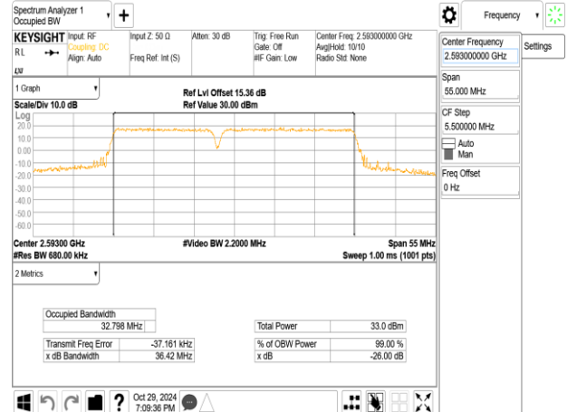
Band41_15MHz+20MHz_QPSK_RB75-0+RB100-0_CH40523+CH40694
