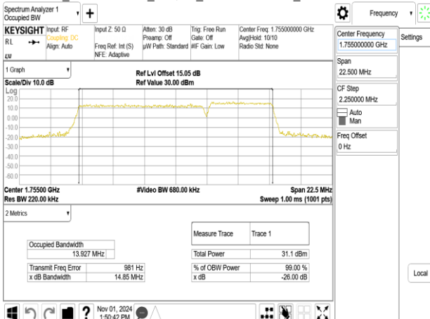
Band66B_10MHz+5MHz_16QAM_RB50-0+RB25-0_CH132397+CH132469
