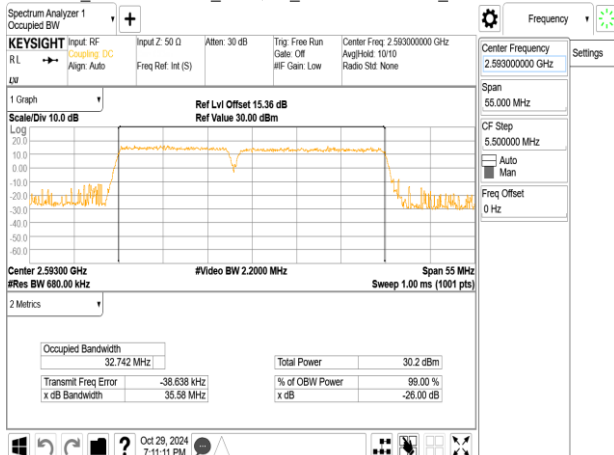
Band41_15MHz+20MHz_256QAM_RB75-0+RB100-0_CH40523+CH40694
