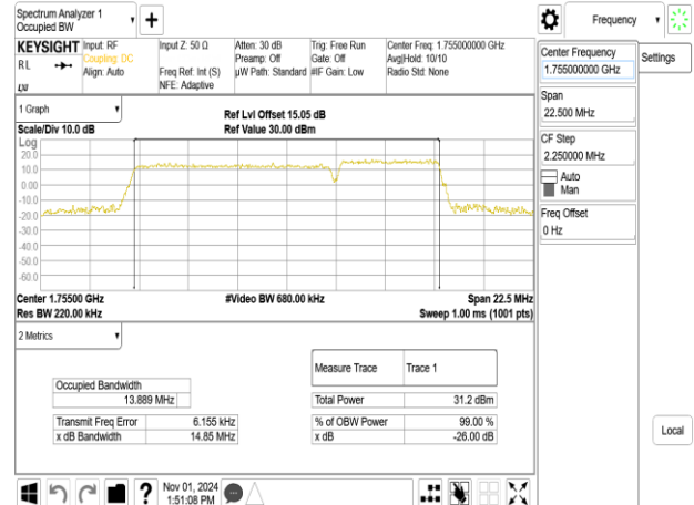
Band66B_10MHz+5MHz_256QAM_RB50-0+RB25-0_CH132397+CH132469
