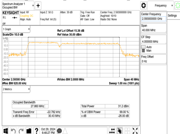
Band41_10MHz+20MHz_256QAM_RB50-0+RB100-0_CH40526+CH40670
