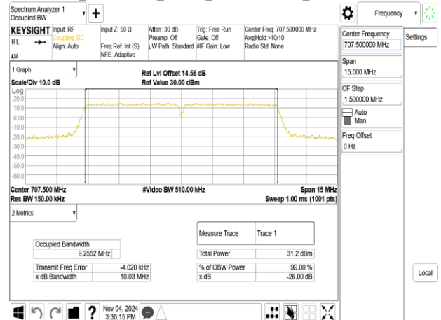
Band12B_5MHz+5MHz_16QAM_RB25-0+RB25-0_CH23071+CH23119
