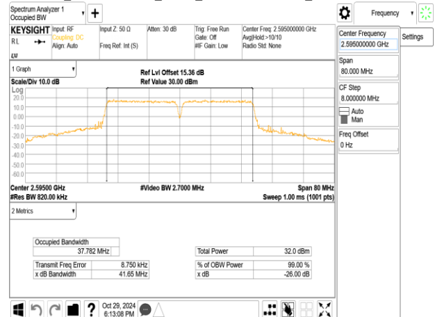
Band38_20MHz+20MHz_QPSK_RB100-0+RB100-0_CH37952+CH38150
