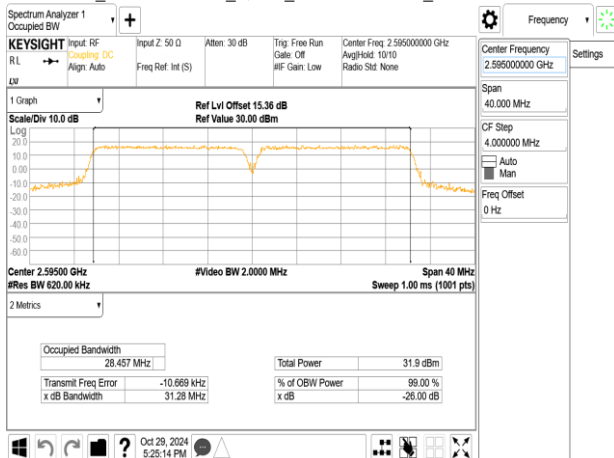
Band38_15MHz+15MHz_16QAM_RB75-0+RB75-0_CH37925+CH38075
