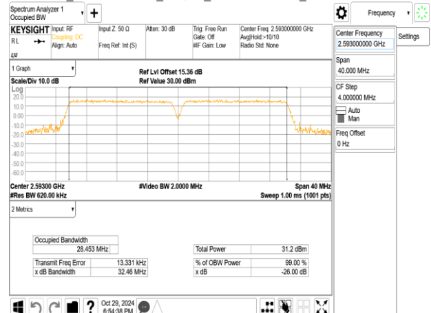
Band41_15MHz+15MHz_64QAM_RB75-0+RB75-0_CH40545+CH40695
