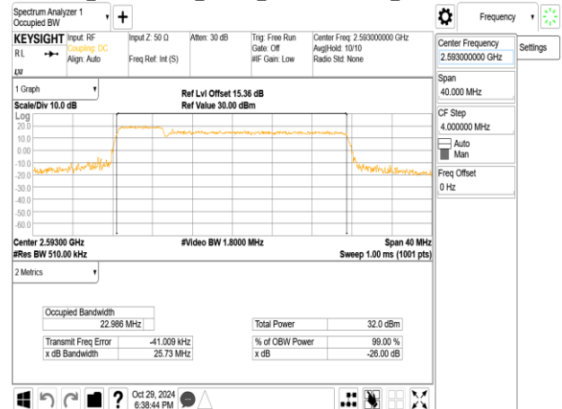
Band41_5MHz+20MHz_64QAM_RB25-0+RB100-0_CH40528+CH40645
