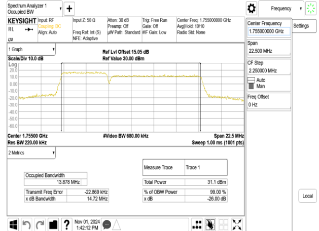
Band66B_5MHz+10MHz_64QAM_RB25-0+RB50-0_CH132375+CH132447
