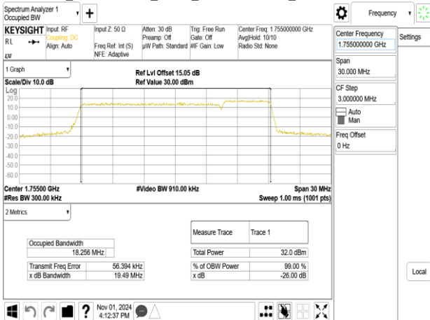
Band66B_15MHz+5MHz_16QAM_RB75-0+RB25-0_CH132398+CH132491
