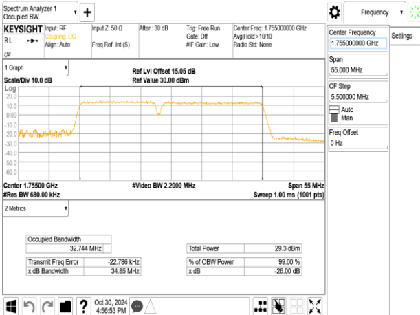
Band66_20MHz+15MHz_QPSK_RB100-0+RB75-0_CH132348+CH132519
