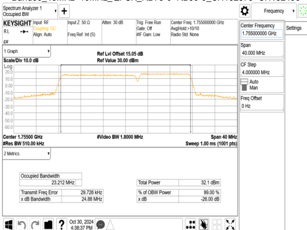
Band66_15MHz+10MHz_16QAM_RB75-0+RB50-0_CH132373+CH132493
