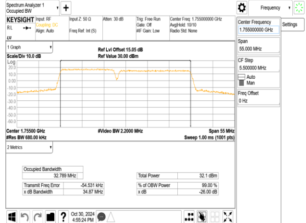
Band66_15MHz+20MHz_16QAM_RB75-0+RB100-0_CH132325+CH132496
