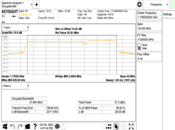
Band66_20MHz+10MHz_64QAM_RB100-0+RB50-0_CH132373+CH132517
