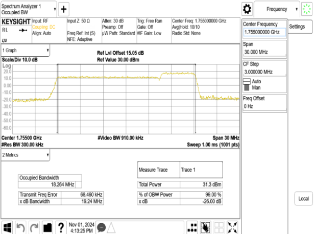
Band66B_15MHz+5MHz_256QAM_RB75-0+RB25-0_CH132398+CH132491
