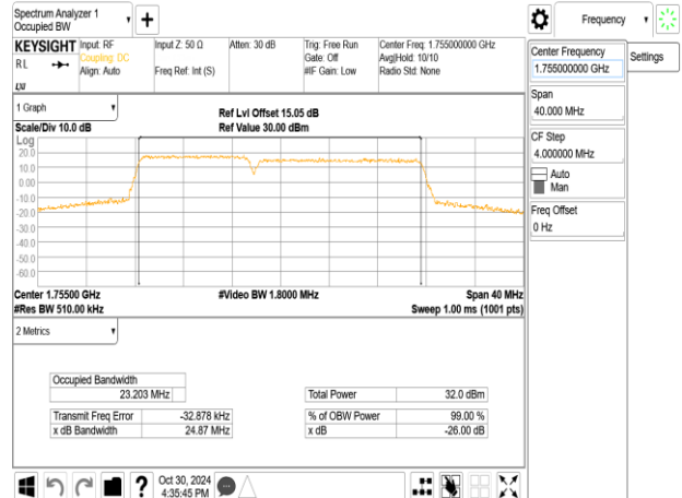
Band66_10MHz+15MHz_16QAM_RB50-0+RB75-0_CH132351+CH132471
