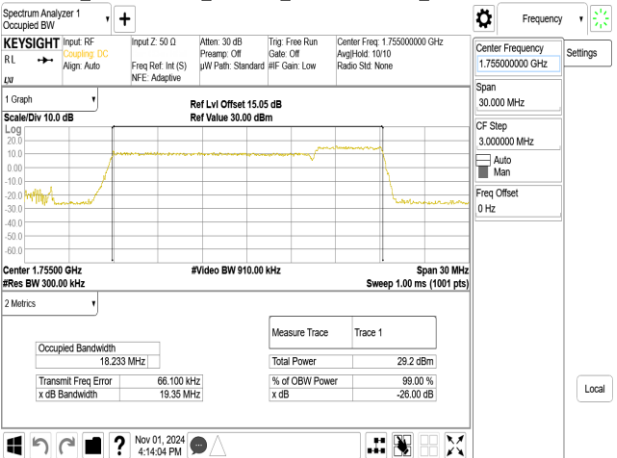
Band66_5MHz+20MHz_QPSK_RB25-0+RB100-0_CH132330+CH132447
