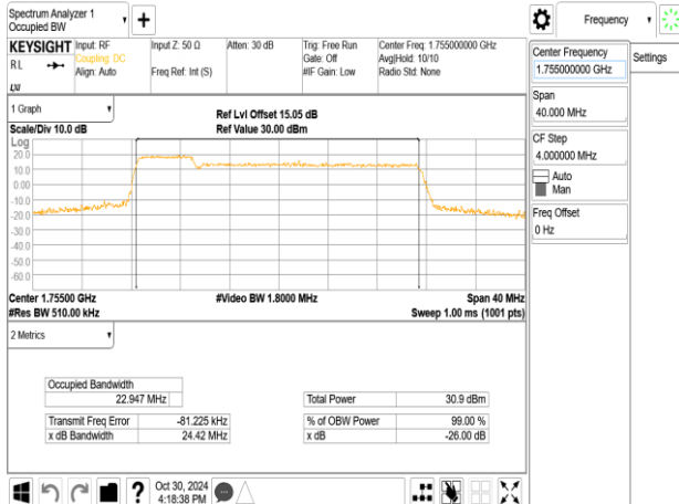
Band66_5MHz+20MHz_64QAM_RB25-0+RB100-0_CH132330+CH132447
