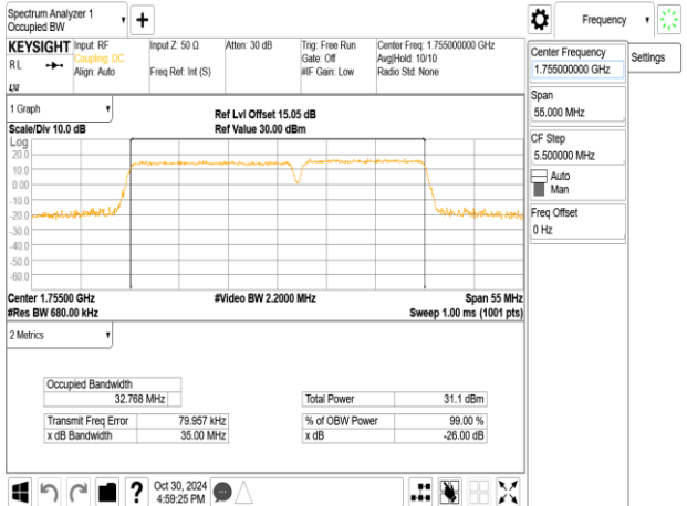
Band66_20MHz+15MHz_256QAM_RB100-0+RB75-0_CH132348+CH132519
