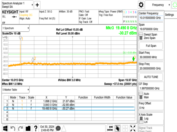
Band2_15MHz+15MHz_QPSK_RB1-74_1-0_CH18975-19125
