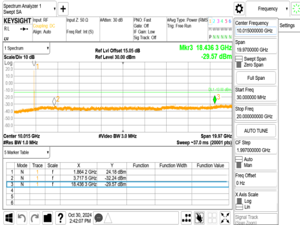
Band2_15MHz+15MHz_QPSK_RB1-74_1-0_CH18825-18975
