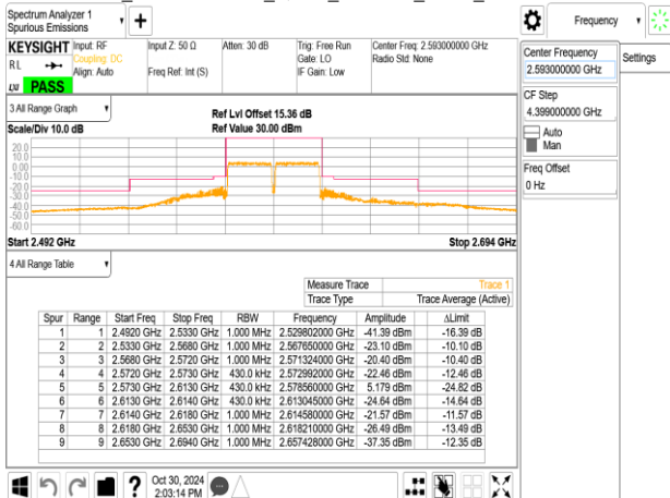
Band41_20MHz+20MHz_QPSK_RB100-0_100-0_CH40521-40719
