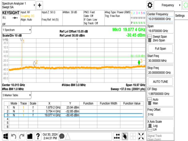
Band2_15MHz+15MHz_QPSK_RB1-74_1-0_CH18975-19125
