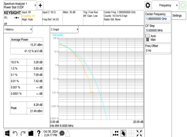
Band2_10MHz+20MHz_256QAM_RB50-0+RB100-0_CH18806+CH18950
