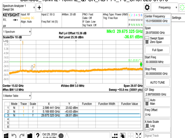
Band38_15MHz+15MHz_QPSK_RB1-74_1-0_CH37925-38075
