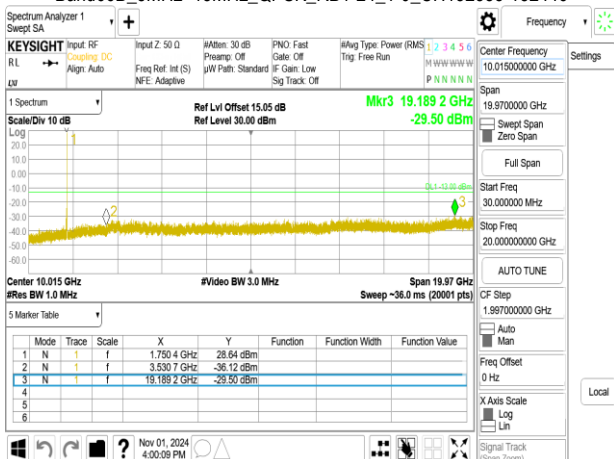
Band66B_5MHz+15MHz_QPSK_RB1-24_1-0_CH132504-132597
