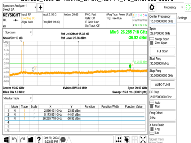
Band38_15MHz+15MHz_QPSK_RB1-74_1-0_CH38025-38175
