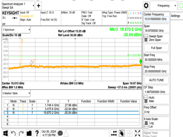
Band66_5MHz+20MHz_QPSK_RB1-24_1-0_CH132455-132572
