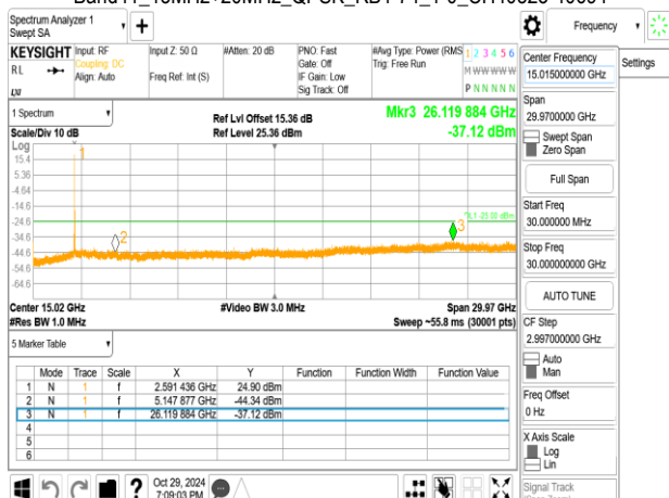
Band41_15MHz+20MHz_QPSK_RB1-74_1-0_CH41319-41490
