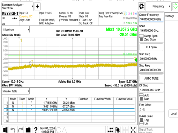
Band66B_5MHz+15MHz_QPSK_RB1-24_1-0_CH132353-132446
