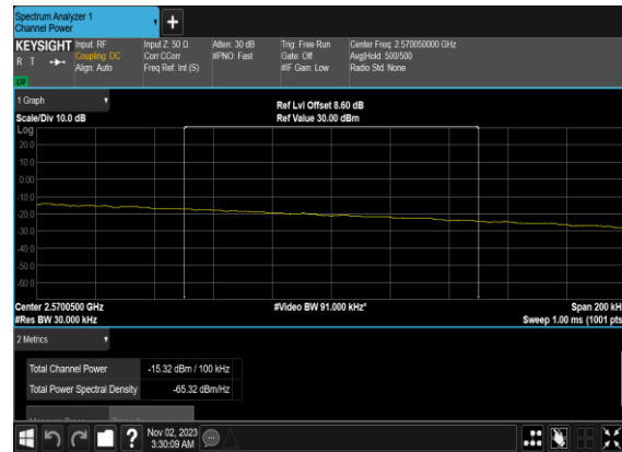
N7(5M)_DFT-s- OFDM_QPSK_Edge_1RB_Right_High_CH_chp_P ASS
