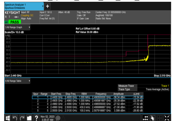
N7(20M)_DFT-s- OFDM_QPSK_Outer_Full_Low_CH
