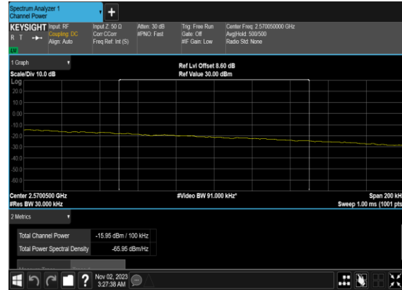
N7(5M)_DFT-s- OFDM_BPSK_Edge_1RB_Right_High_CH_chp_P ASS
