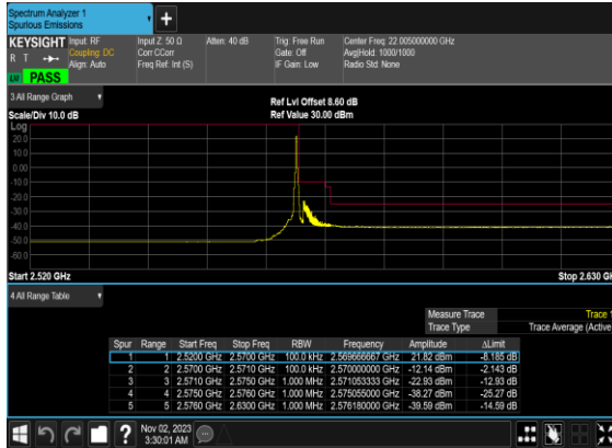
N7(5M)_DFT-s- OFDM_QPSK_Edge_1RB_Right_High_CH
