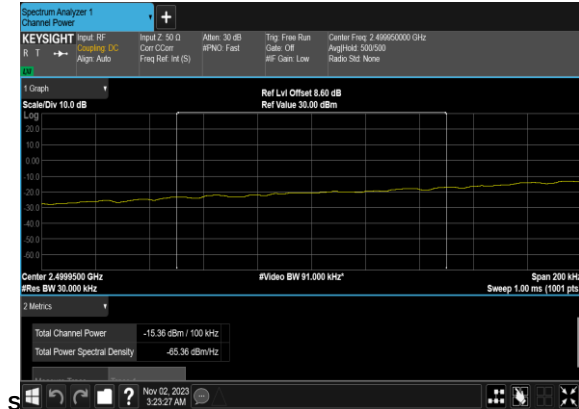
N7(5M)_DFT-s- OFDM_QPSK_Edge_1RB_Left_Low_CH_CHP_PAS
