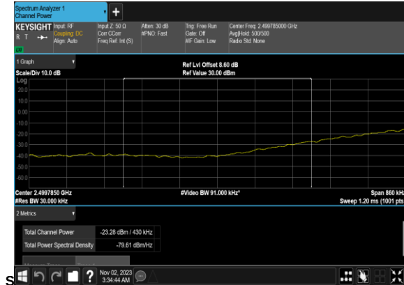
N7(20M)_DFT-s- OFDM_QPSK_Edge_1RB_Left_Low_CH_CHP_PAS
