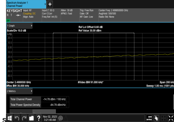
N7(5M)_DFT-s- OFDM_BPSK_Edge_1RB_Left_Low_CH_CHP_PAS
