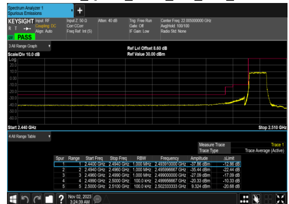
N7(5M)_DFT-s- OFDM_QPSK_Outer_Full_Low_CH
