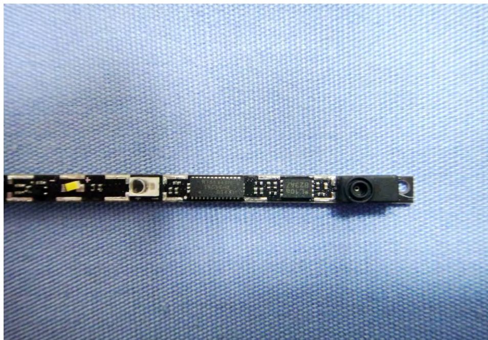
EUT Photo (80)
