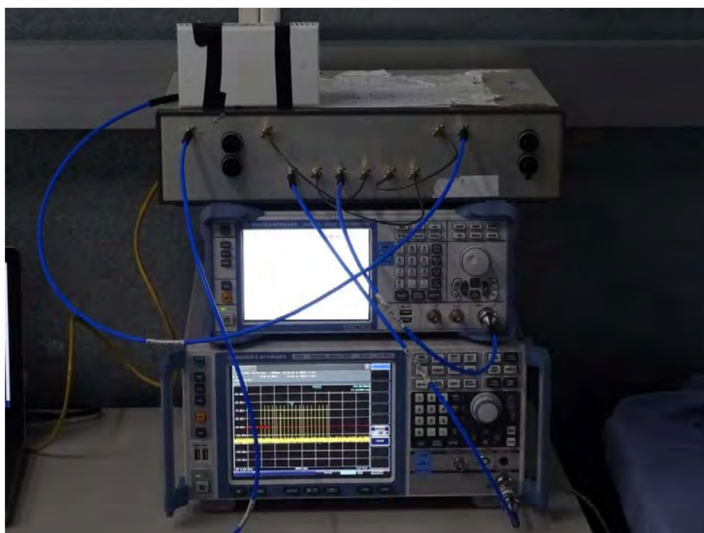
DFS Test Setup Photo: Master and Spectrum Analyzer and Radar Generator
