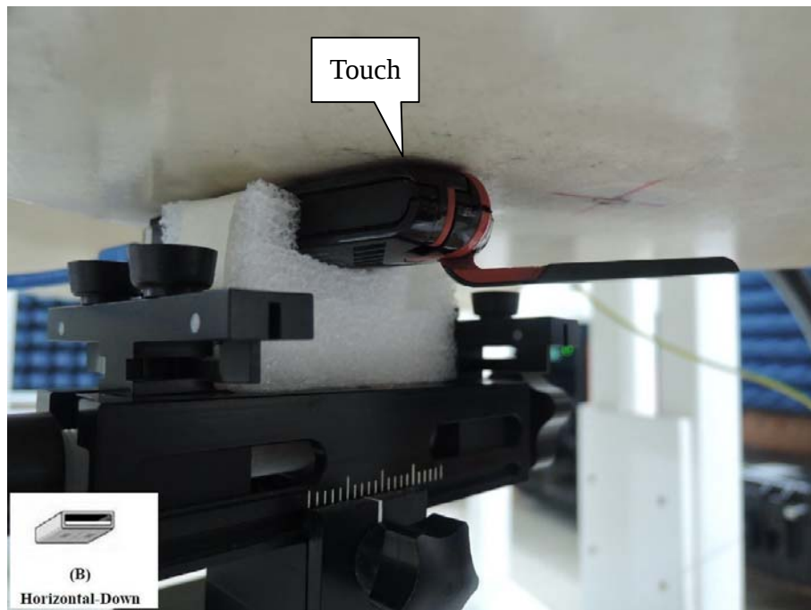
EUT Front (TX1 Antenna Position: 180° )
