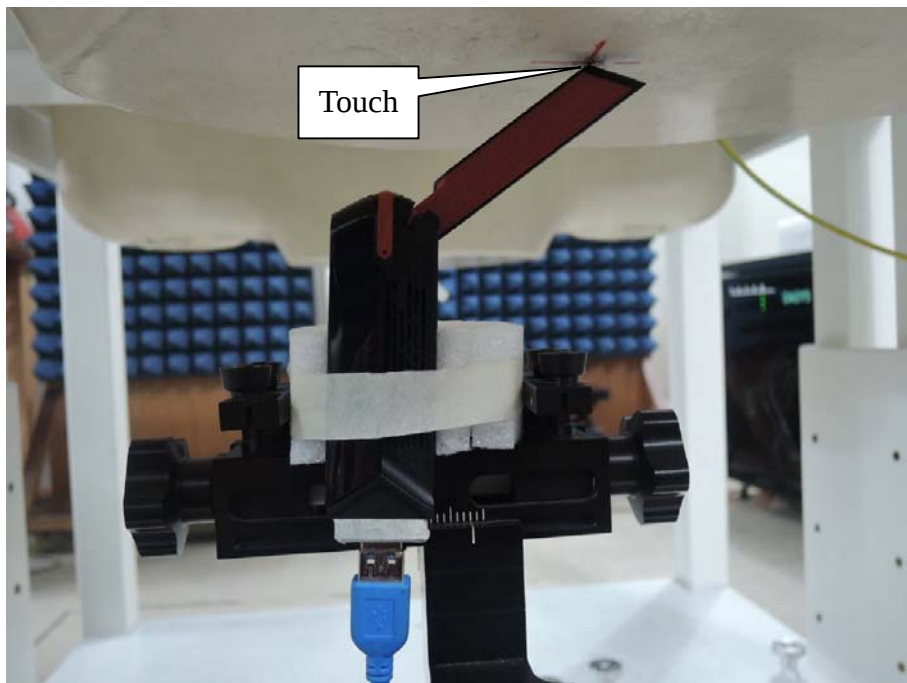
EUT Tip (TX3 Antenna Position: 180° )
