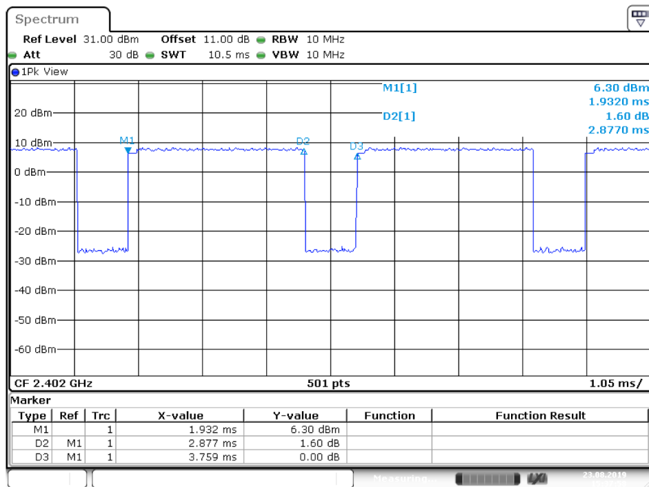
Time-domain plot for Bluetooth transmission signal
