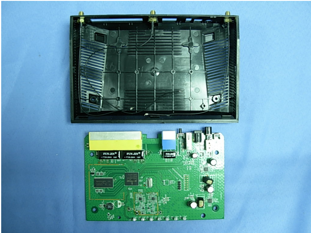
(11) EUT Photo
