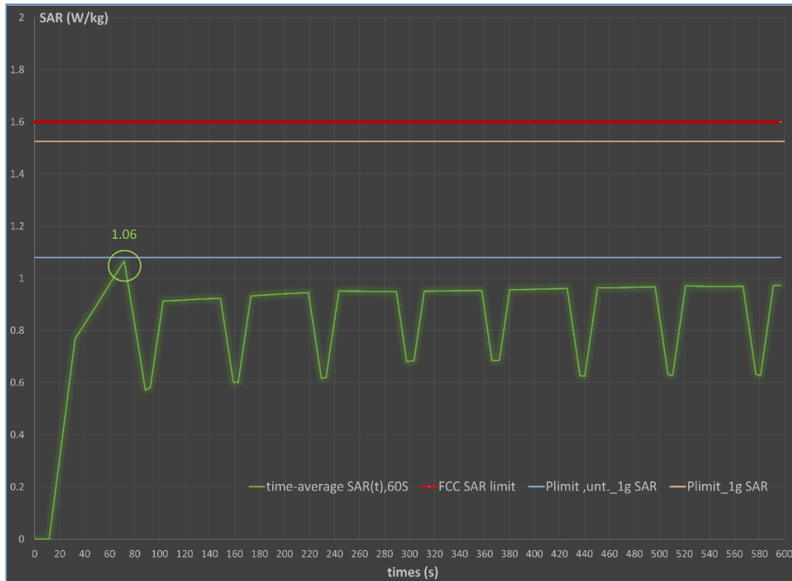
Figure 6-3: Time-Averaged SAR Over Time for Test Scenario 1
