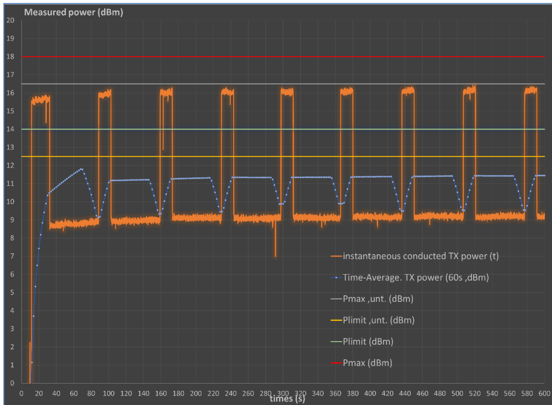
Figure 6-2: Time-Averaged Conducted Tx Power Over Time for Test Scenario 1
