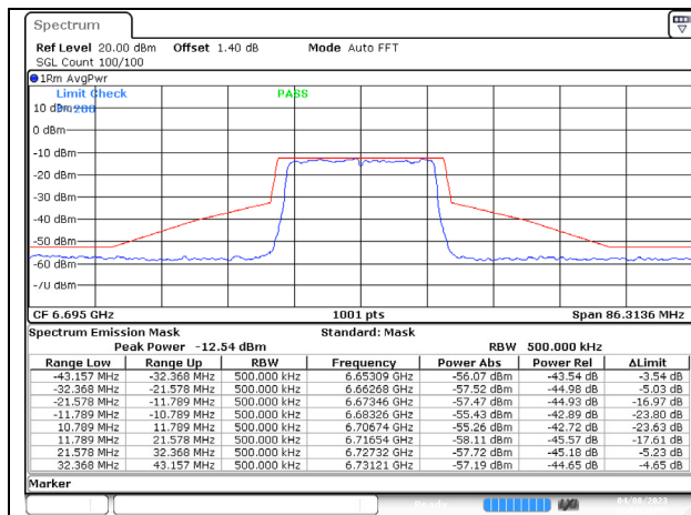
802.11ax (20MHz) 6695MHz Chain C NSS-1
