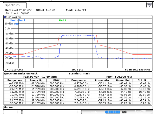
802.11ax (20MHz) 7015MHz Chain B NSS-1
