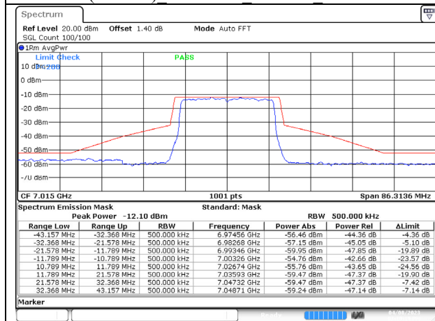
802.11ax (20MHz) 7015MHz Chain A NSS-1
