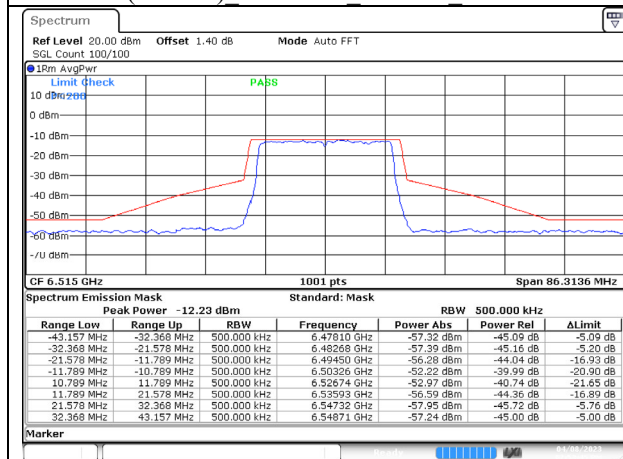
802.11ax (20MHz) 6515MHz Chain A NSS-1
