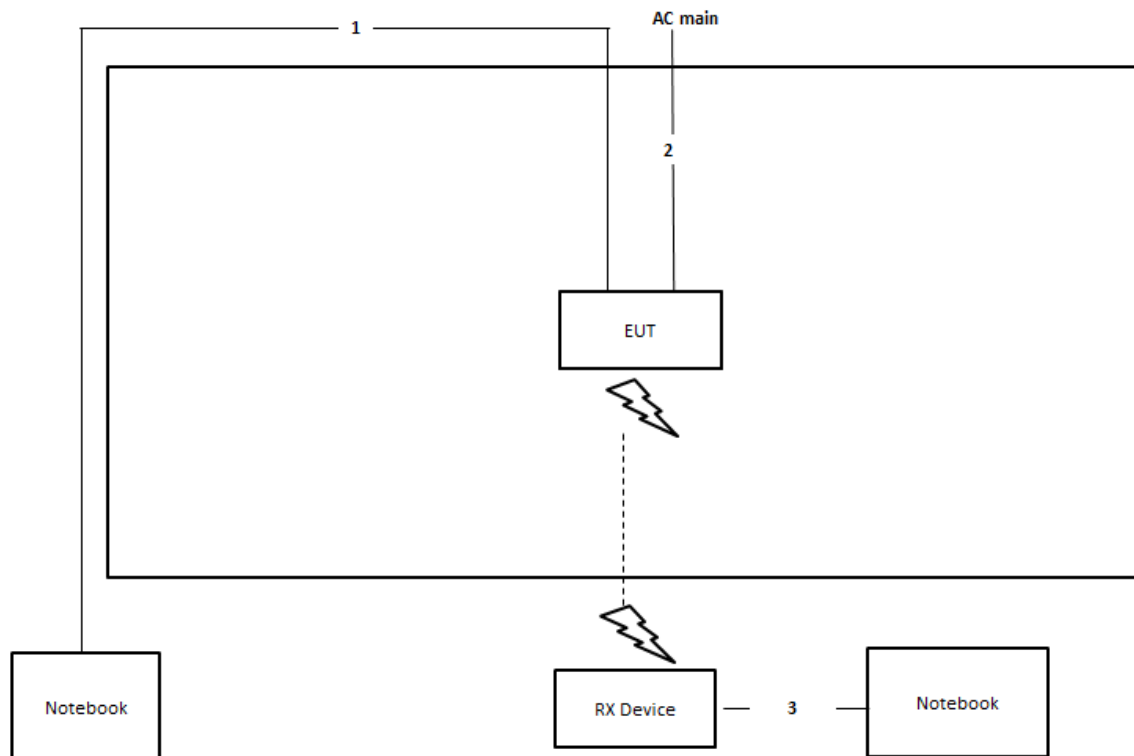
Test Setup Diagram - Radiated Test (Above 1GHz) For beamforming mode
