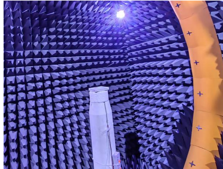
2D/3D Radiation pattern test
