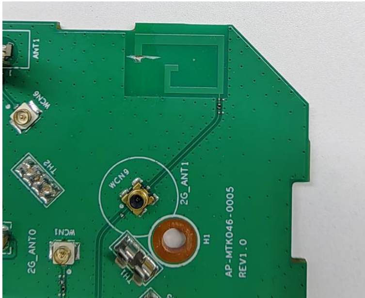
2G Antenna
