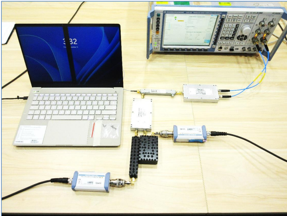
Setup for Conducted Power Testing (Simultaneous Transmission)
