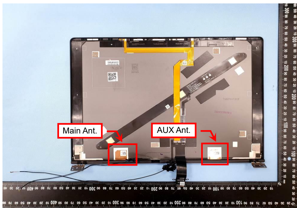
EUT Photo (22)
