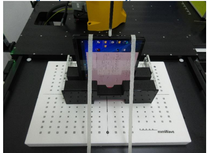
Testing Setup for Power Density, Left Side at 0 mm
