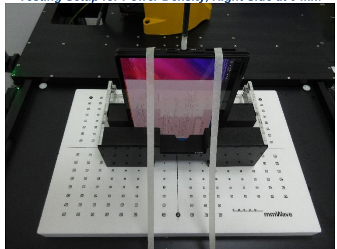
Testing Setup for Power Density, Right Side at 0 mm
