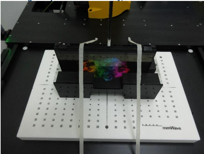
Testing Setup for Power Density, Bottom Side at 0 mm
