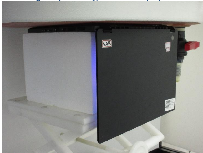
Testing Setup for Body, Bottom of Laptop at 0 mm
