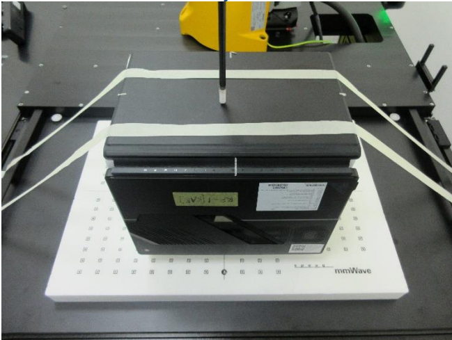
Testing Setup for Power Density, Back of Display Screen at 25 mm, w/ Keyboard
