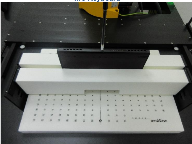
Testing Setup for Power Density, Top Side at 0 mm, w/o Keyboard
