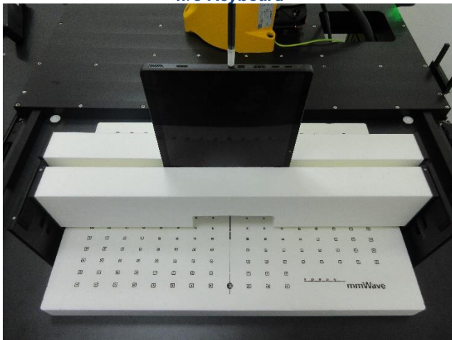
Testing Setup for Power Density, Left Side at 0 mm, w/o Keyboard
