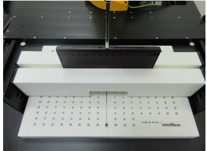
Testing Setup for Power Density, Bottom Side at 0 mm, w/o Keyboard
