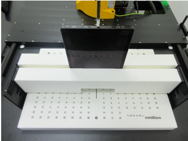
Testing Setup for Power Density, Right Side at 0 mm, w/o Keyboard
