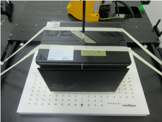
Testing Setup for Power Density, Bottom of Laptop at 0 mm, w/ Keyboard
