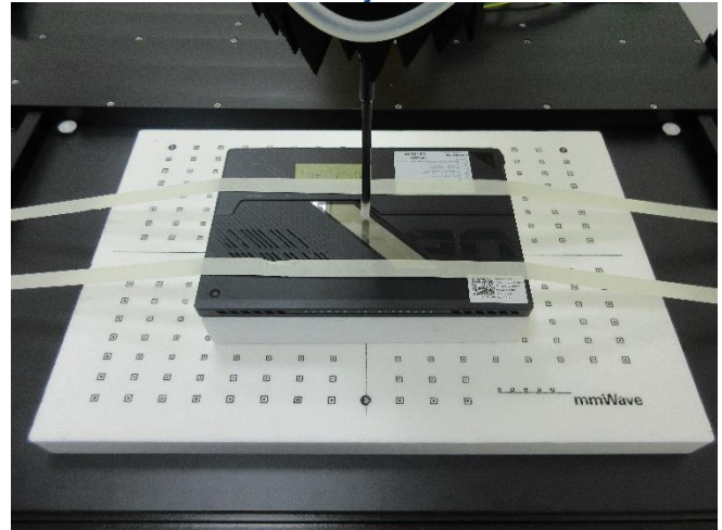
Testing Setup for Power Density, Bottom Surface at 0 mm, w/o Keyboard
