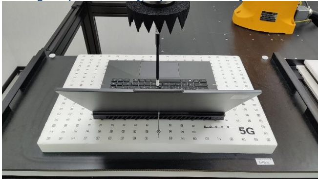
Testing Setup for Extremity, Top Side of the Keyboard at 2 mm
