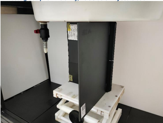
Testing Setup for Extremity, Left Side of keyboard at 0 mm
