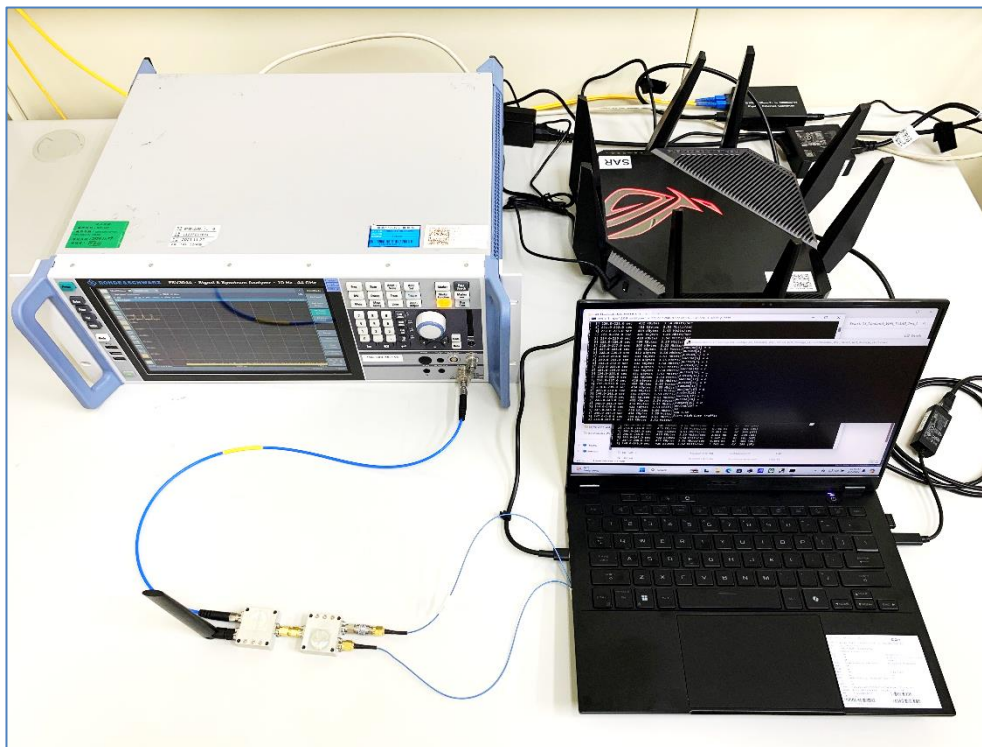
Setup for Conducted Power Testing (Test Scenario 3)
