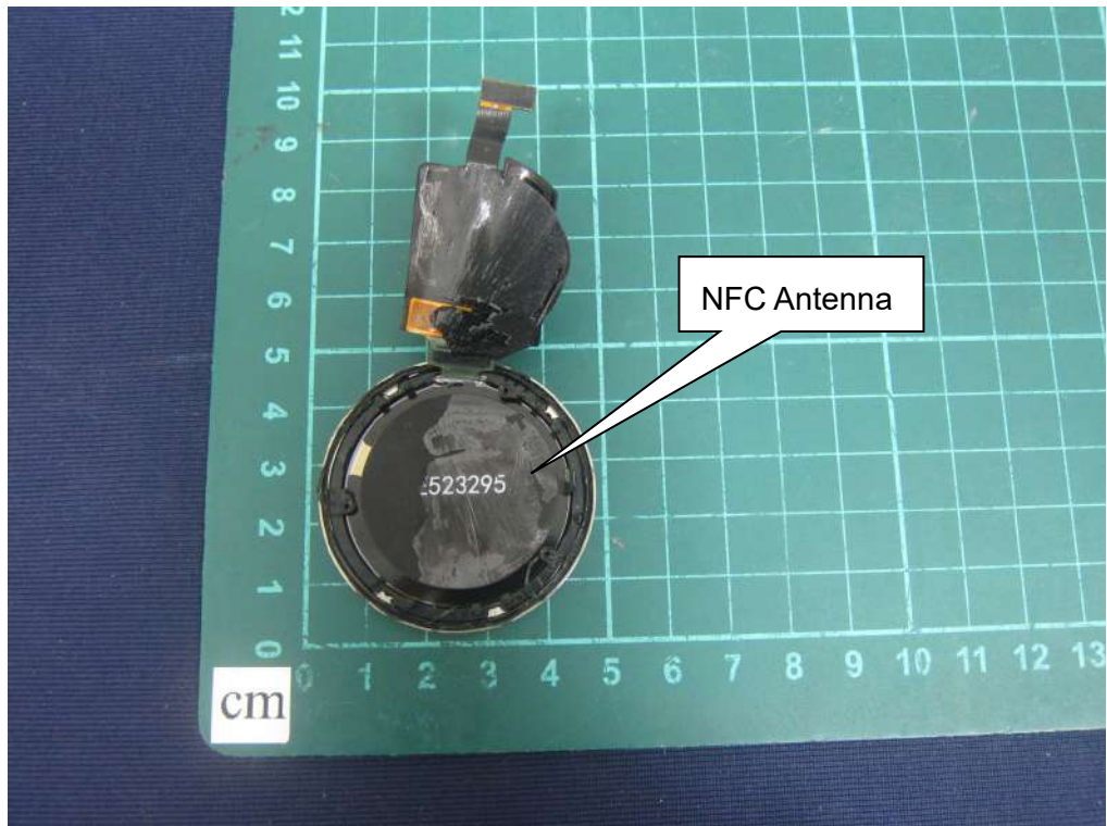
(25) EUT Photo
