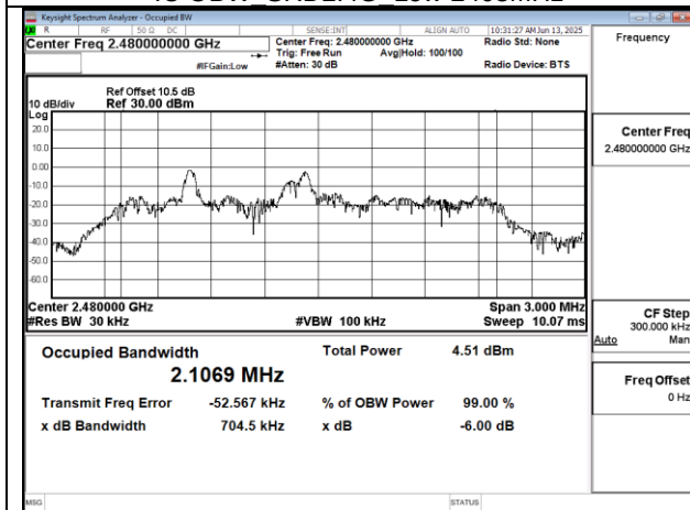
IC OBW_SRD2.4G_High-2480MHz
