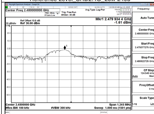
Reference Level SRD2.4G High-2480
