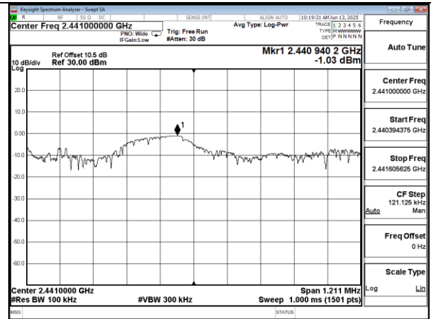
Reference Level SRD2.4G Mid-2441
