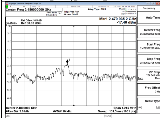
Power Density SRD2.4G High-2480
