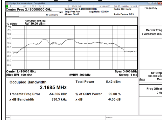
OBW 6dB SRD2.4G High-2480
