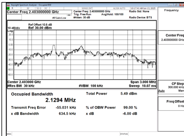
IC OBW_SRD2.4G_Low-2403MHz
