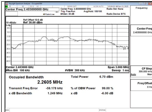
OBW 6dB SRD2.4G Low-2403
