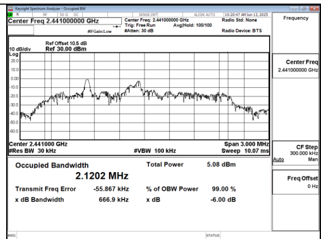
IC OBW_SRD2.4G_Mid-2441MHz
