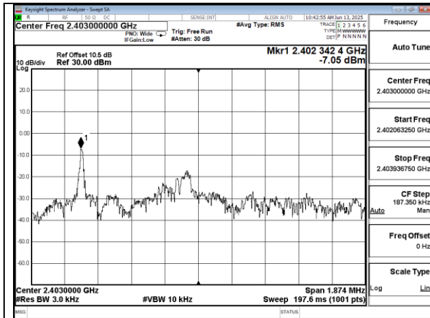
Power Density SRD2.4G Low-2403
