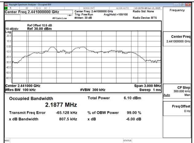
OBW 6dB SRD2.4G Mid-2441
