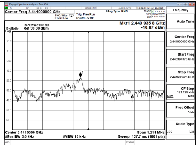
Power Density SRD2.4G Mid-2441
