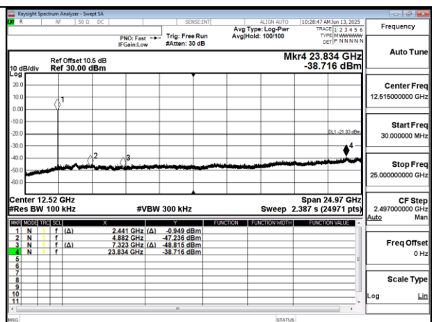
Spurious Emission SRD2.4G Mid-2441
