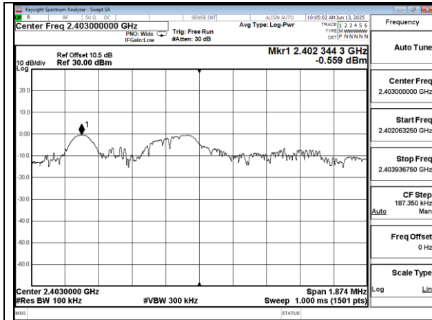
Reference Level SRD2.4G Low-2403
