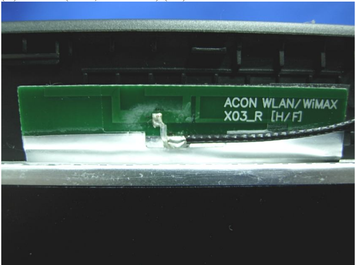
(18) EUT Photo (ACON, APP6P-700432)- (Aux)
