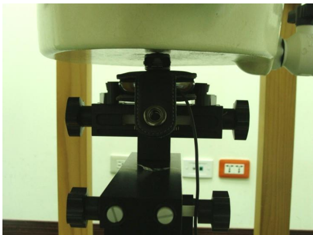
Face of the DUT with Phantom 0 cm Gap With the Holster and Earphone
