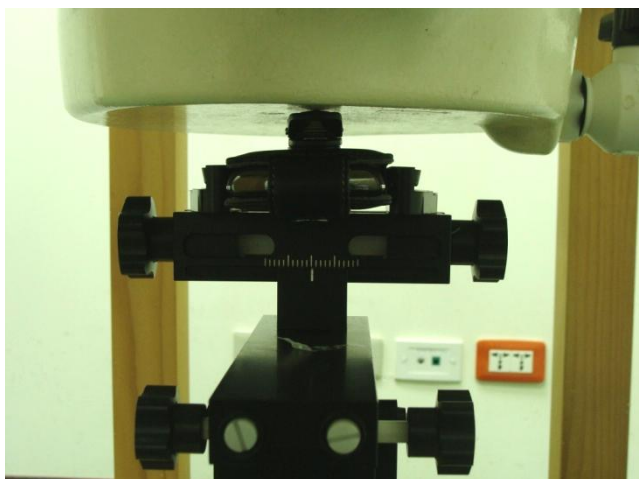
Bottom of the DUT with Phantom 0 cm Gap With the Holster only
