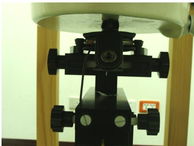
Bottom of the DUT with Phantom 0 cm Gap With the Holster and Earphone
