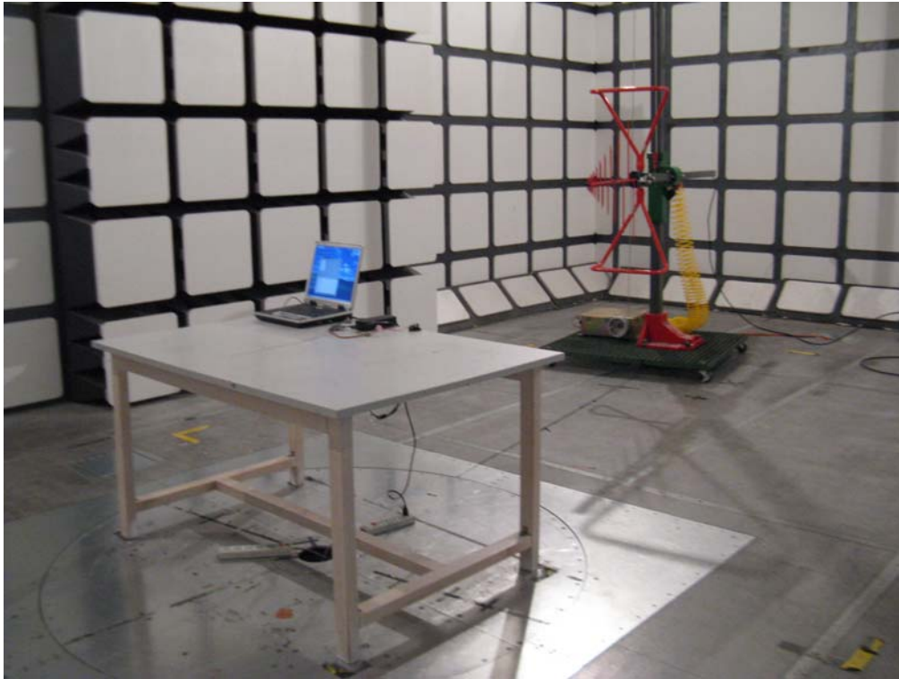
Below 1GHz: Radiated Emissions - Front View (Transmitting Mode)
