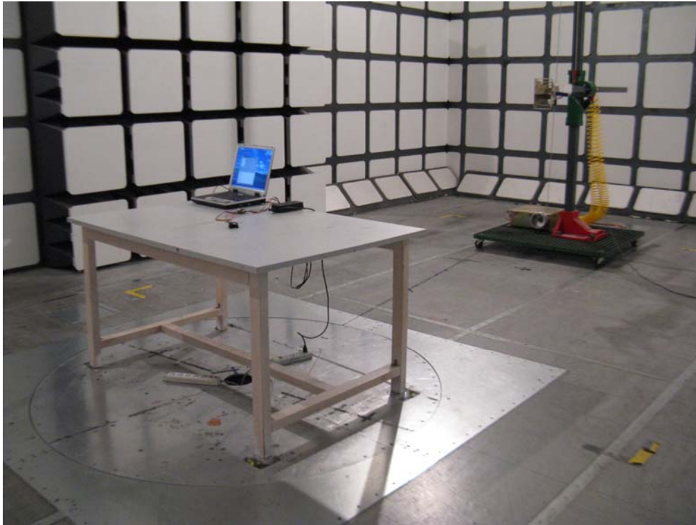
Above 1GHz: Radiated Emissions - Front View (Transmitting Mode)
