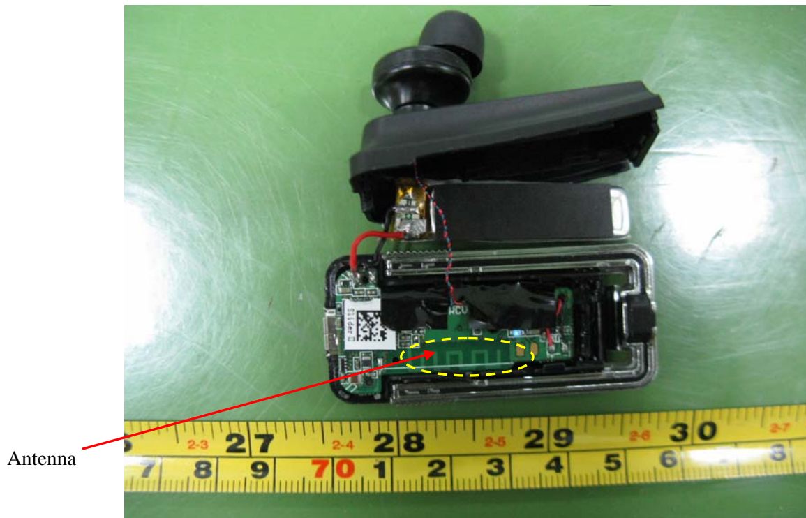
EUT – Cover off View
