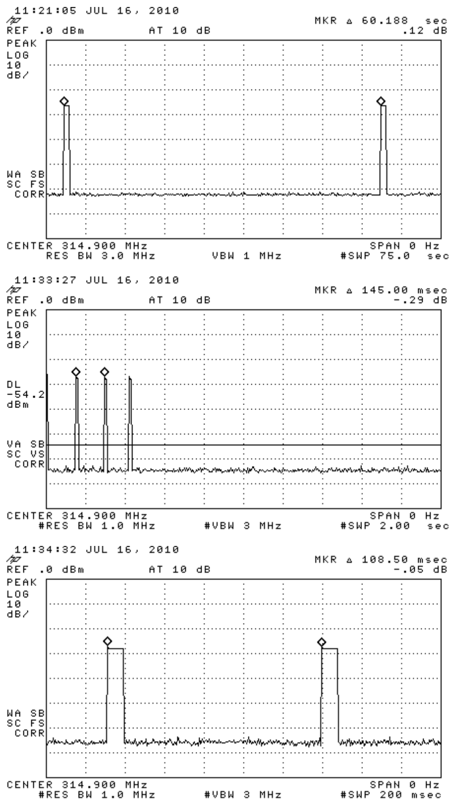
Figure 6.1. Transmission modulation characteristics. (top) drive mode FSK periodic transmission, (center) expanded FSK transmission, (bottom) minimum FSK word separation.
