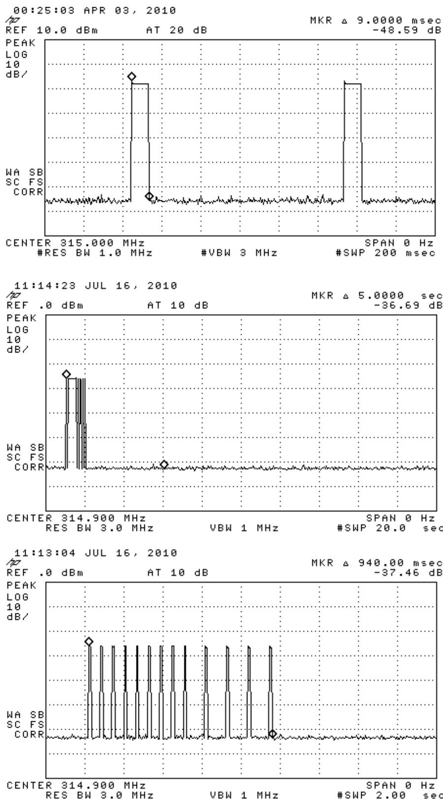
Figure 6.1. Transmission modulation characteristics. (top) FSK word length, (center) LF activated ASK + FSK transmission, (bottom) expanded transmission.
