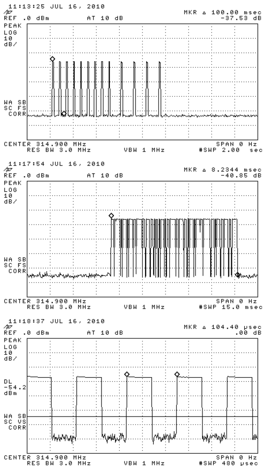
Figure 6.1. Transmission modulation characteristics. (top) two ASK words per 100 ms window, (center) expanded ASK word, (bottom) expanded ASK Manchester encoding.
