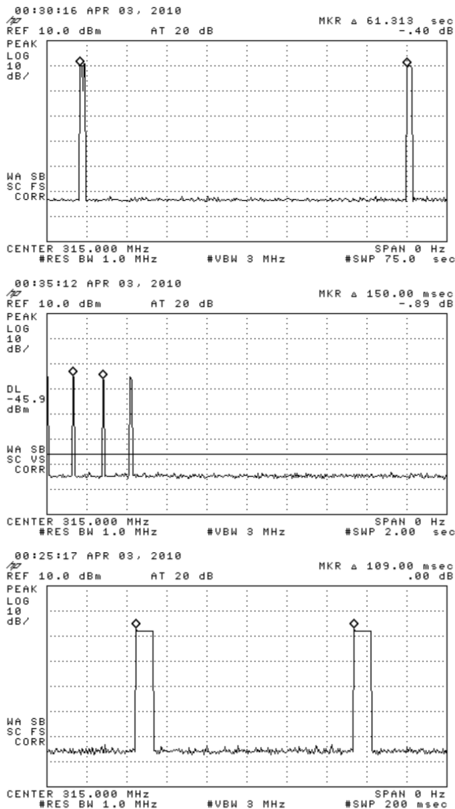
Figure 6.1. Transmission modulation characteristics. (top) drive mode FSK periodic transmission, (center) expanded FSK transmission, (bottom) minimum FSK word separation.
