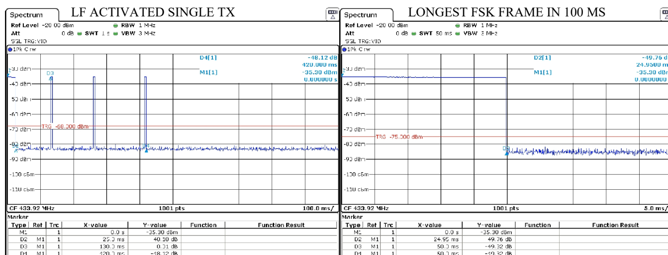
Figure 5(a): Fundamental Emission Pulsed Operation.
