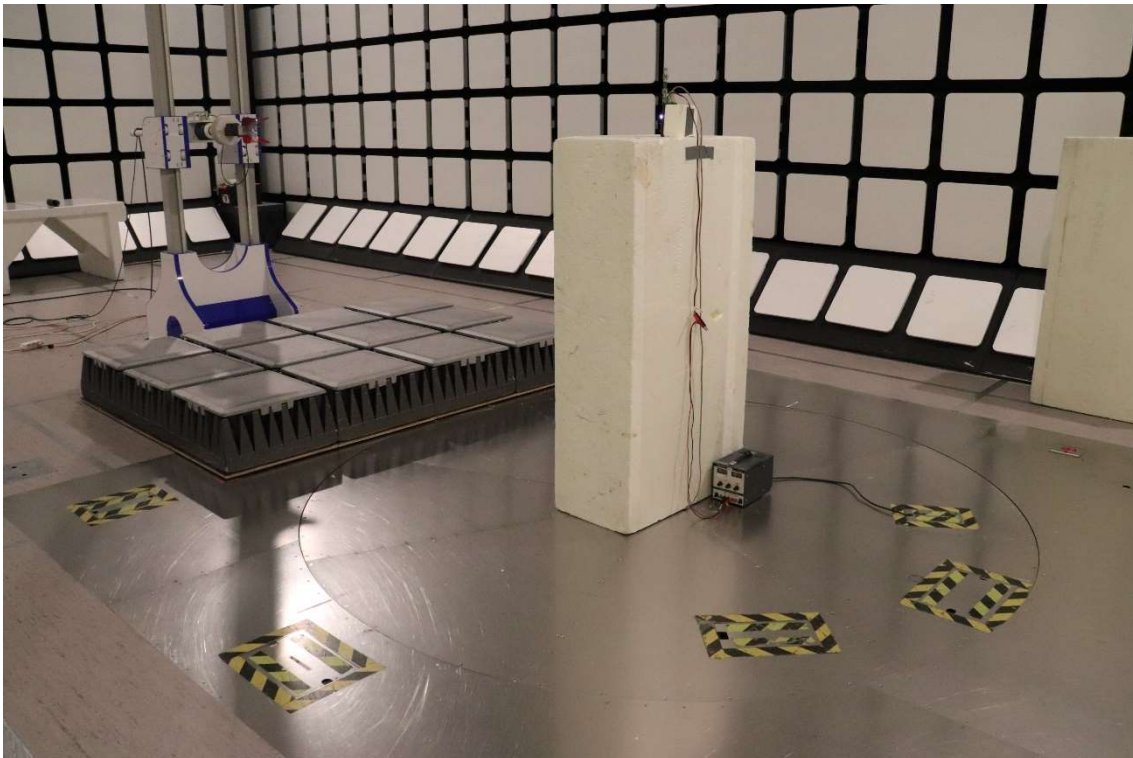
Photograph 3. Radiated Emissions 1 – 5 GHz
