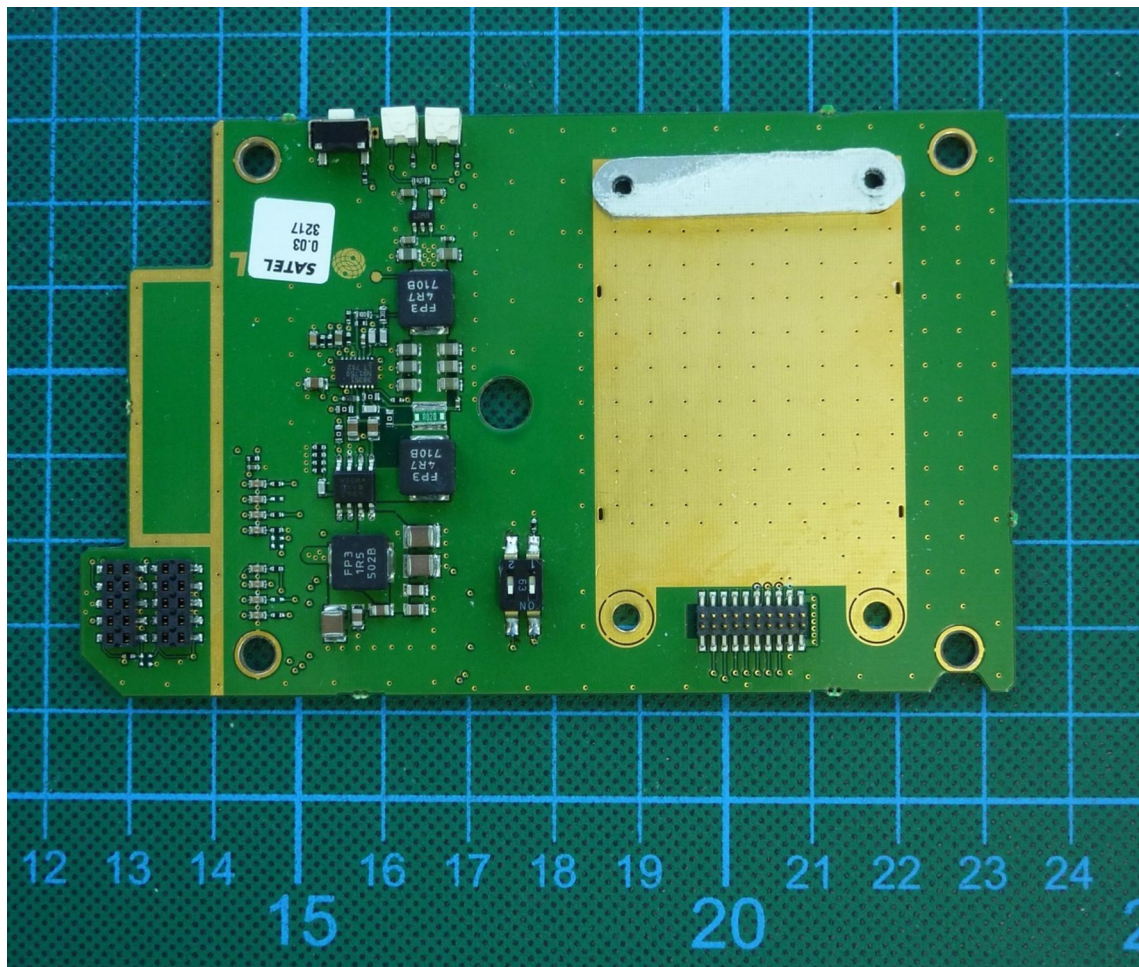
172629_12.jpg: Evaluation board – top view
