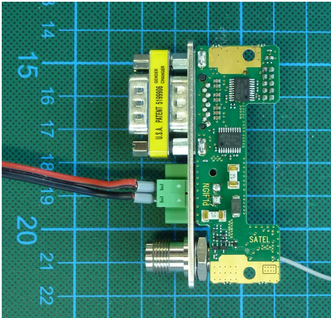
172629_15.jpg: Interface board – bottom view
