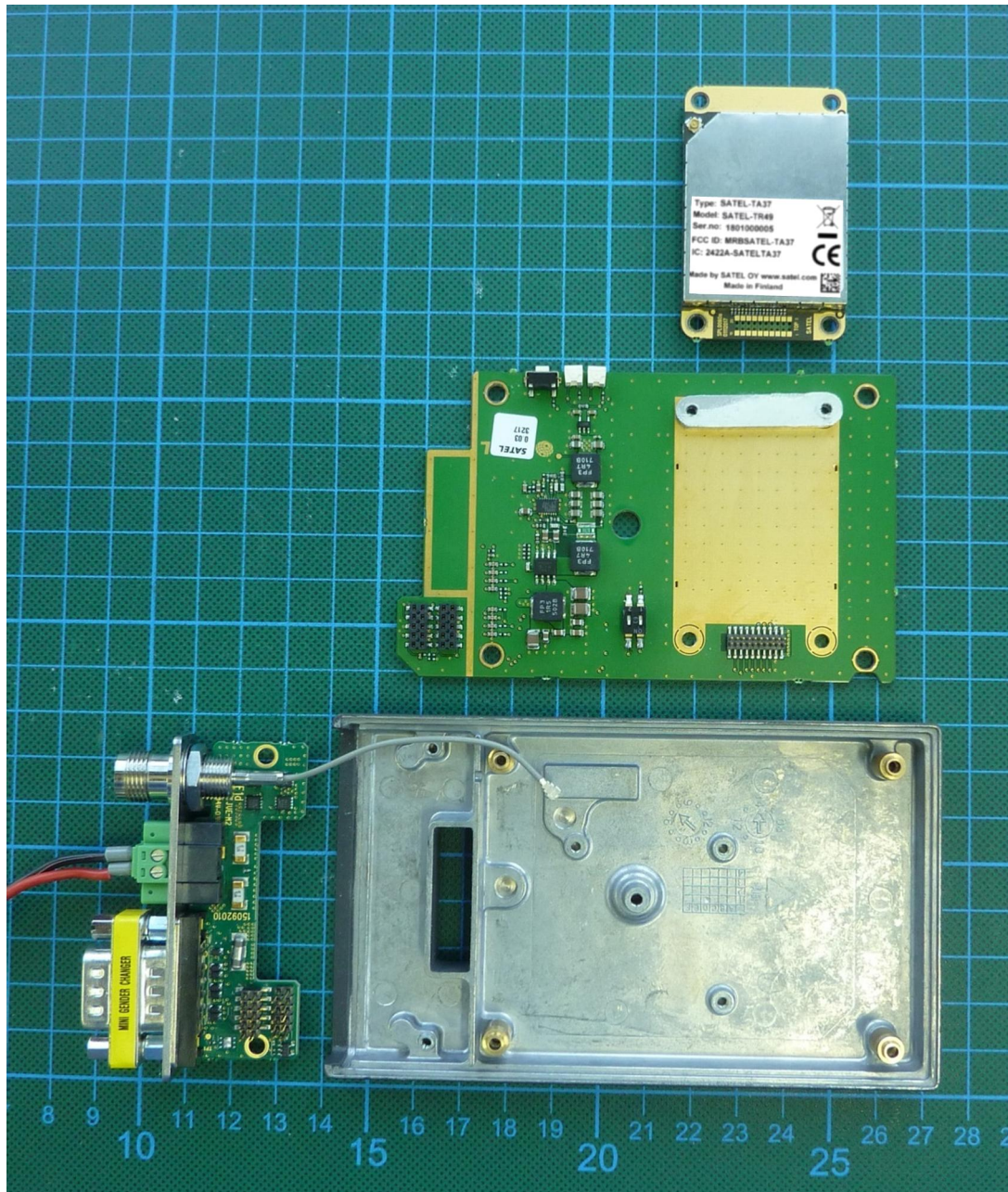
172629_09.jpg: EUT, evaluation board, interface board, housing
