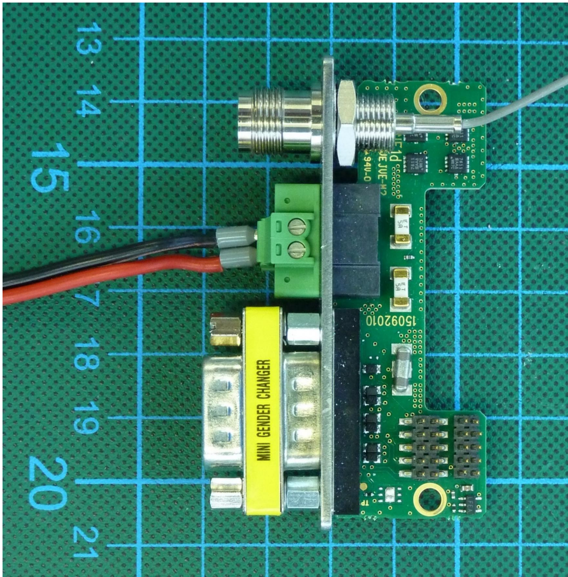
172629_14.jpg: Interface board – top view
