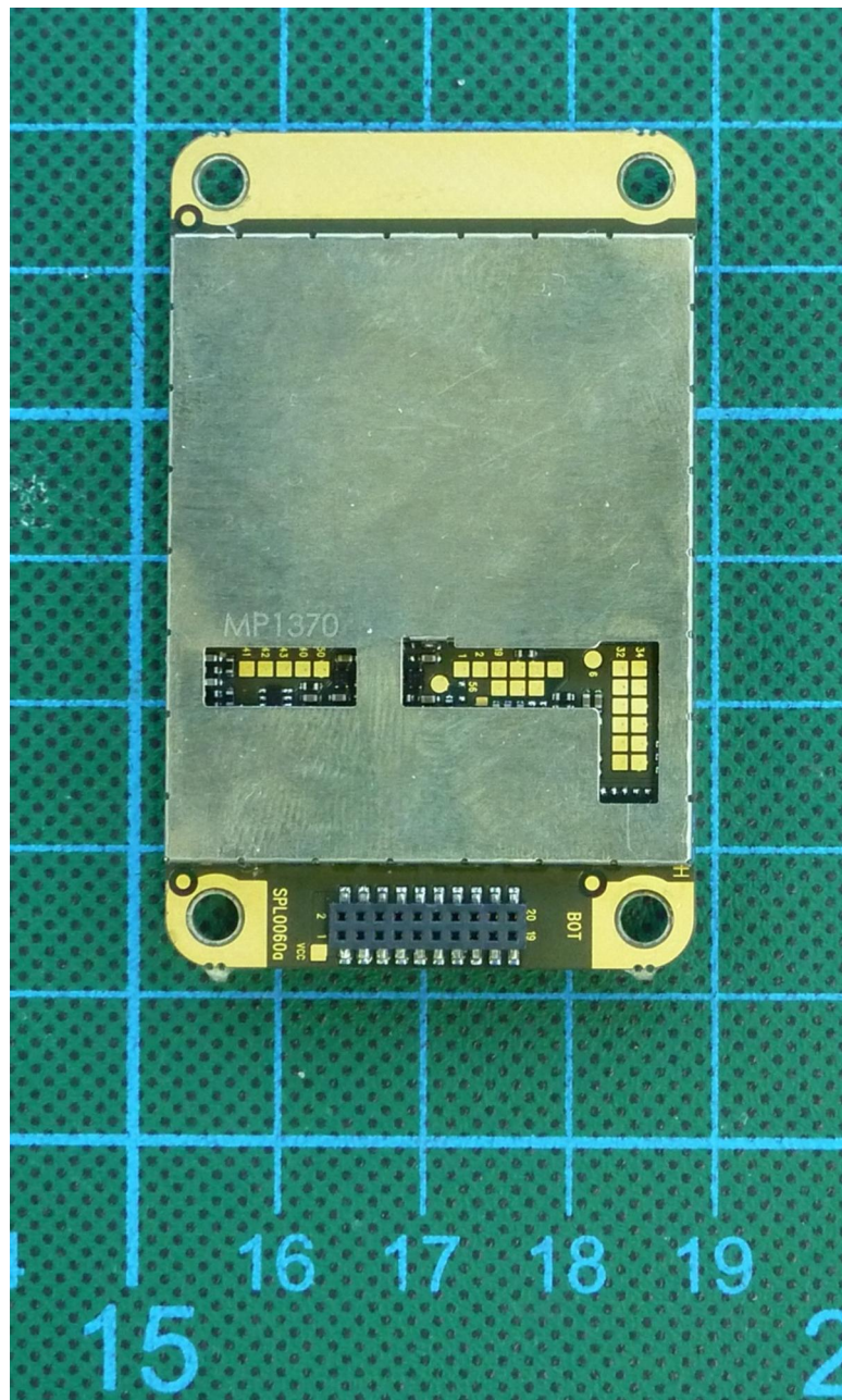
172629_07.jpg: EUT – bottom view
