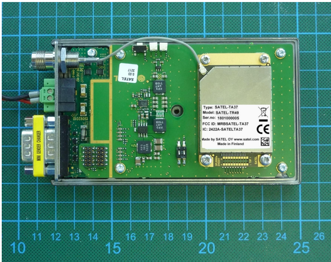
172629_05.jpg: EUT at eval board board
