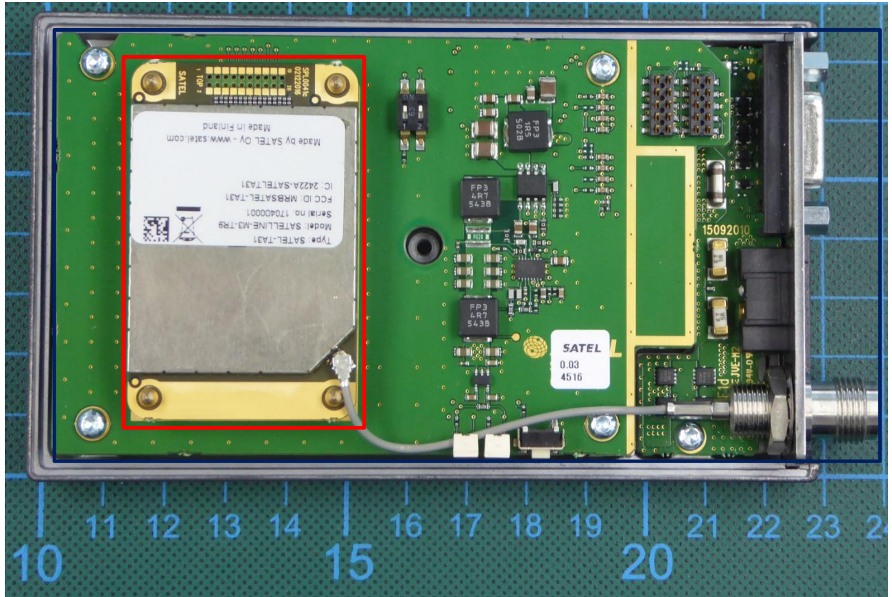
170226_20.jpg: EUT (red) on Eval board (blue) – top view
