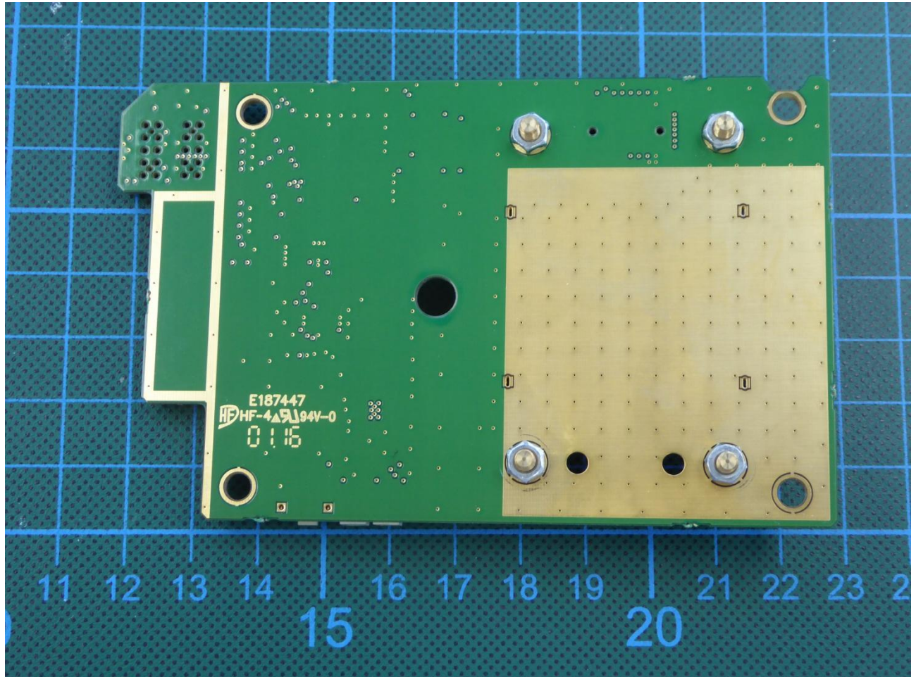
170226_26.jpg: Evalboard – bottom view
