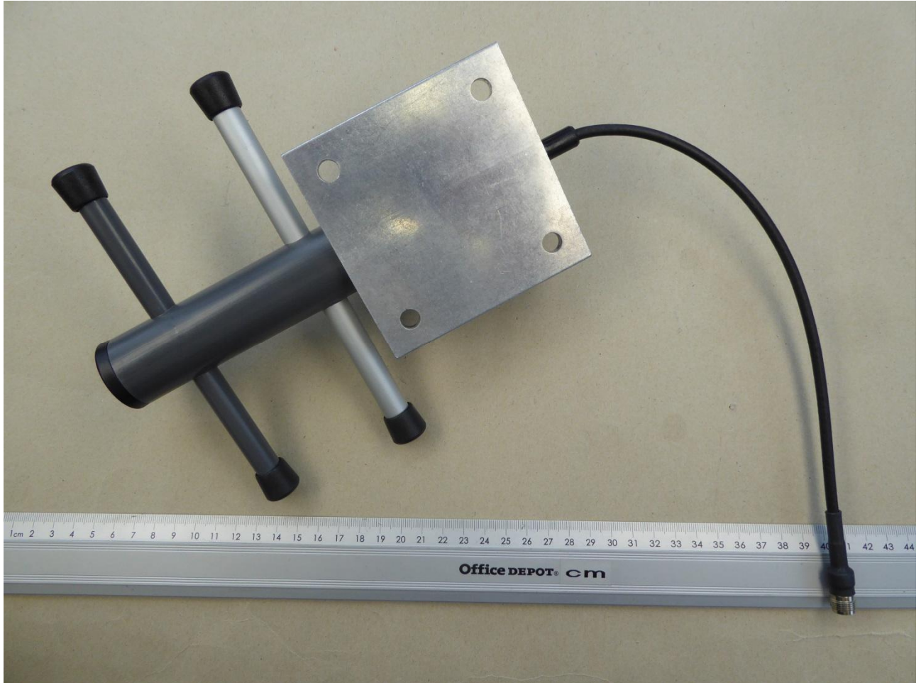
170226_34.jpg: CAY antenna – bottom view
