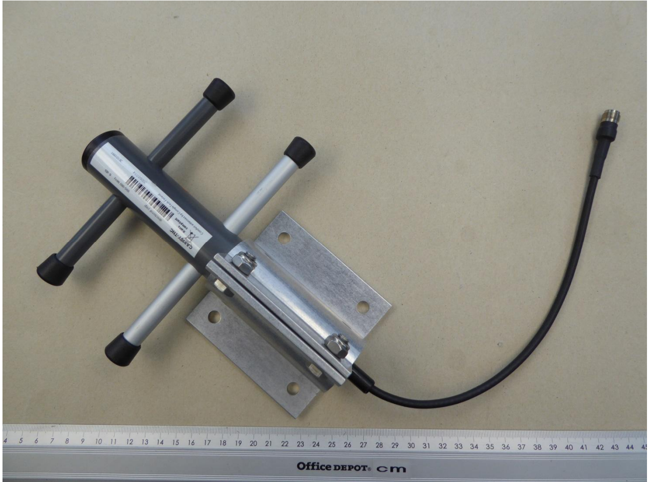
170226_33.jpg: CAY antenna – top view
