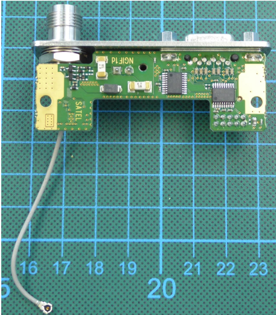
170226_28.jpg: connector board – bottom view
