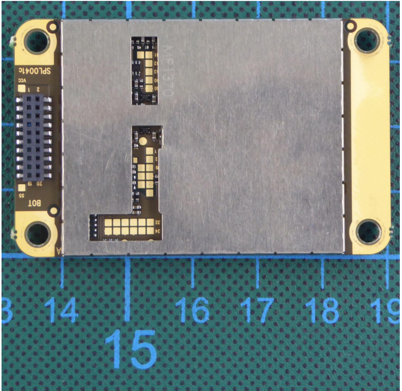
170226_30.jpg: EUT – bottom view
