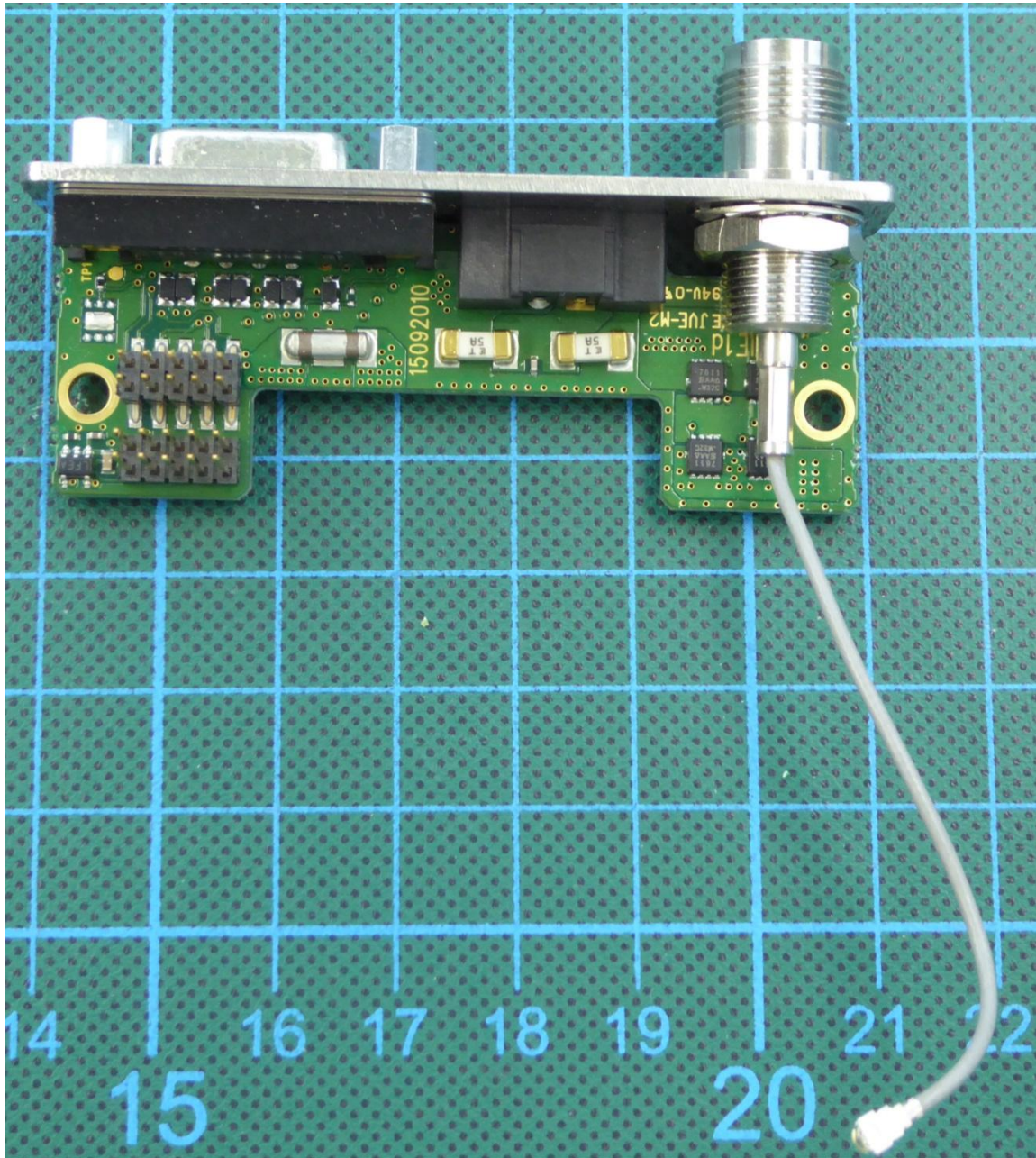
170226_27.jpg: connector board – top view
