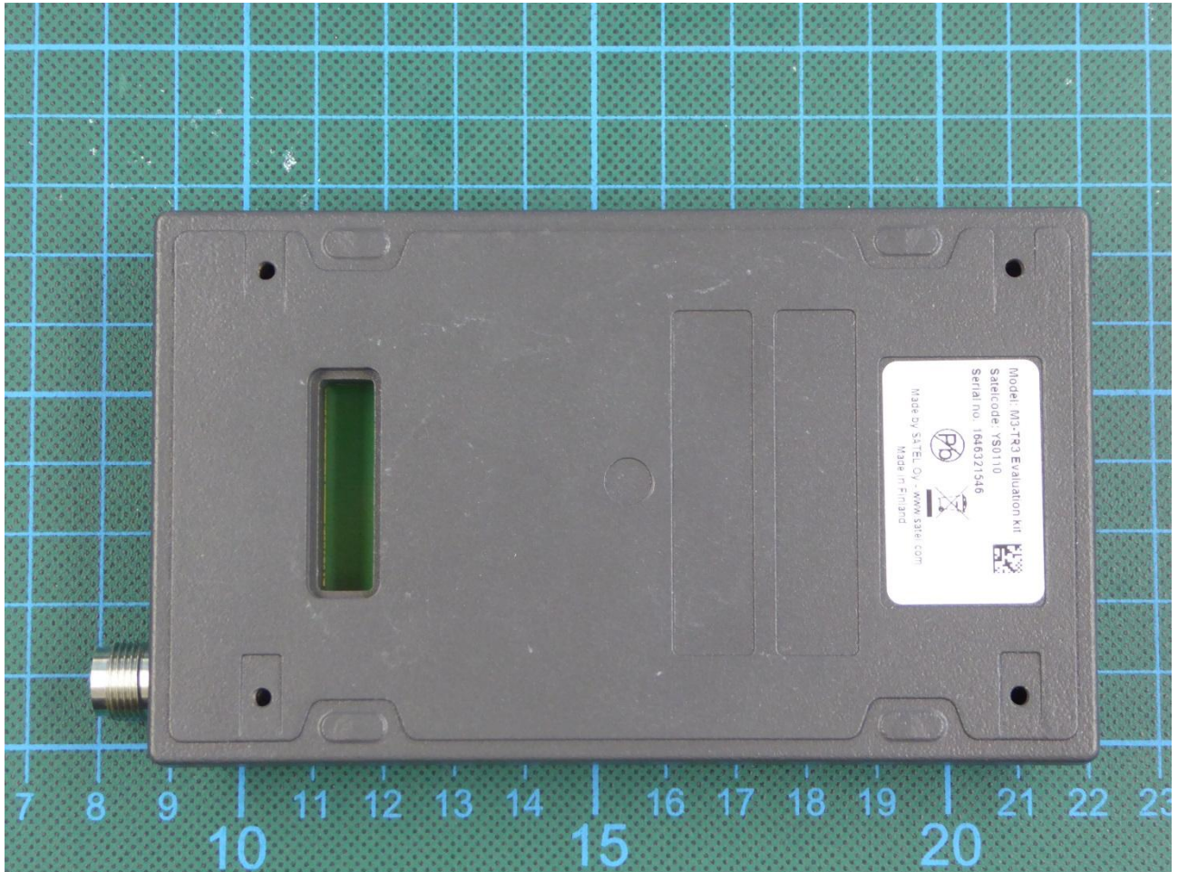
170226_21.jpg: Evalboard housing – bottom view
