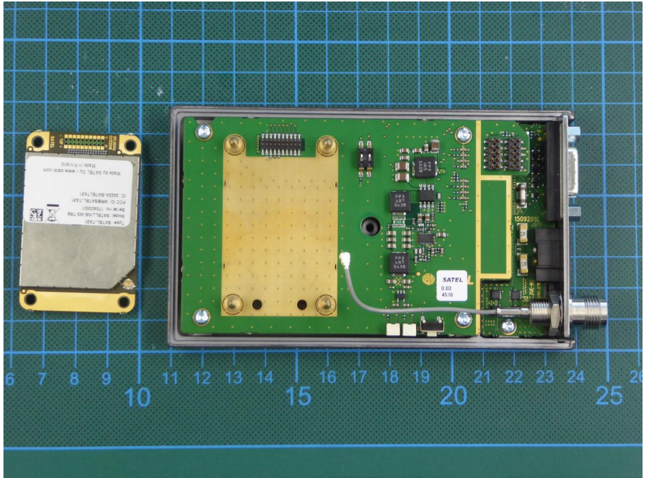
170226_24.jpg: Evalboard housing without EUT – top view
