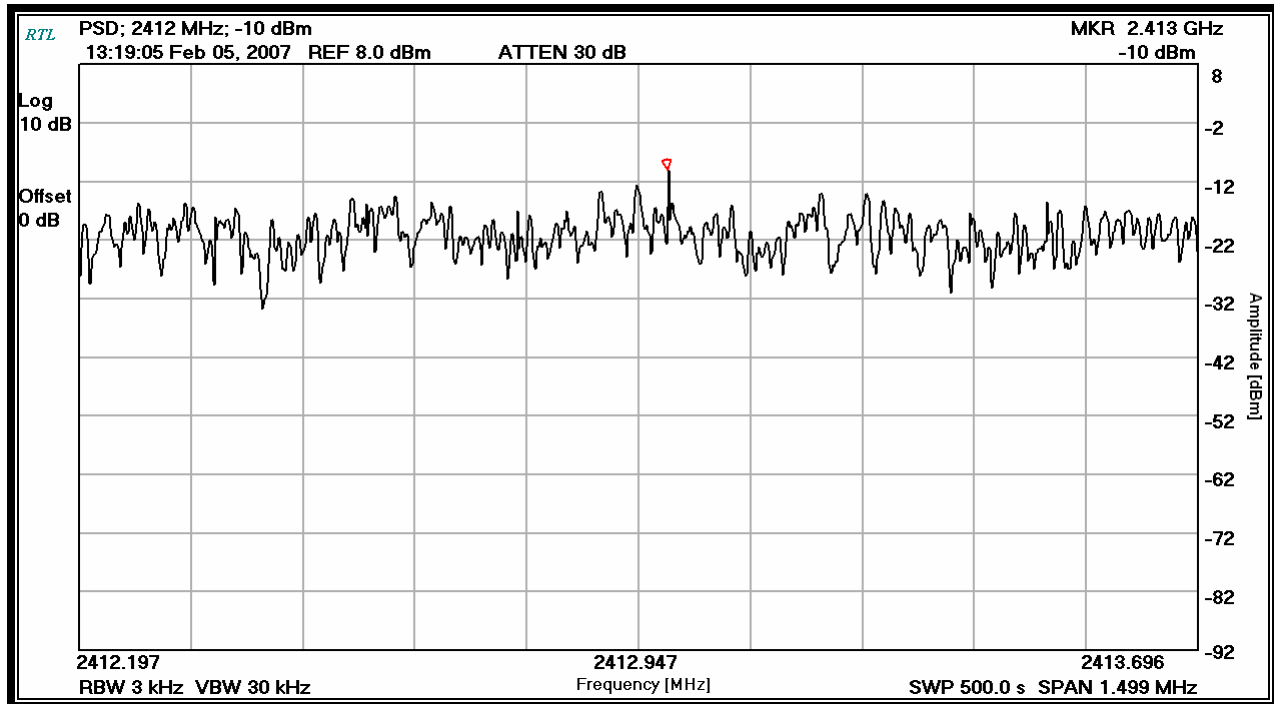
Plot 7-1: Power Spectral Density: Channel 1 (2412 MHz)
