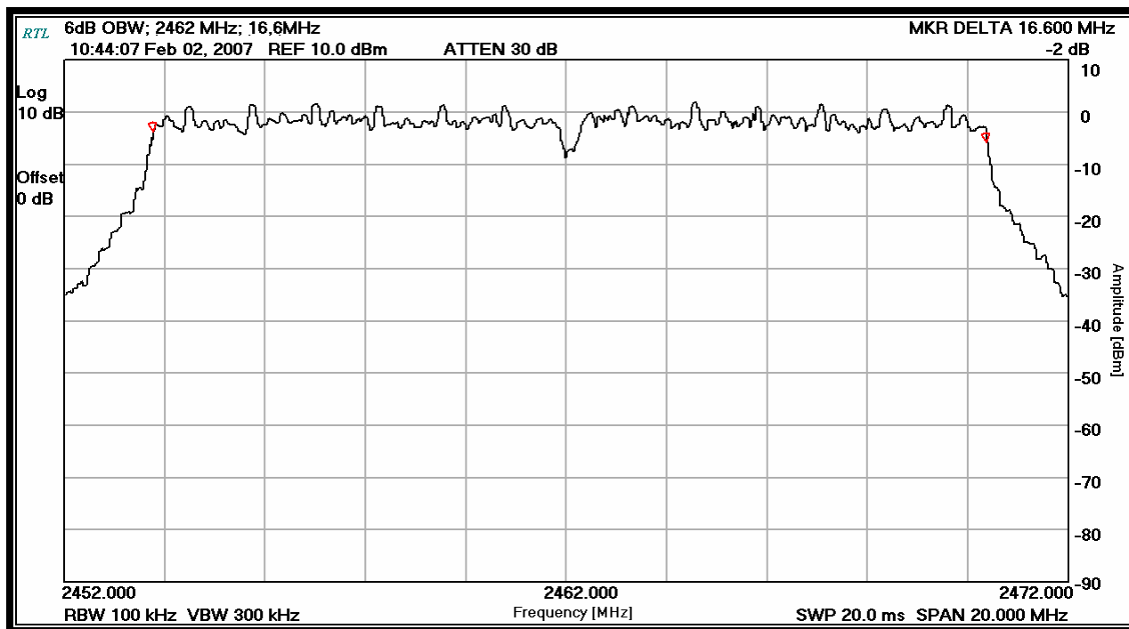
Plot 6-3: 6 dB Bandwidth Channel 11 (TX Frequency: 2462 MHz)
