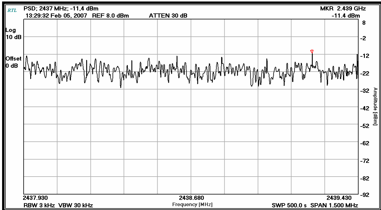
Plot 7-2: Power Spectral Density: Channel 6 (2437 MHz)
