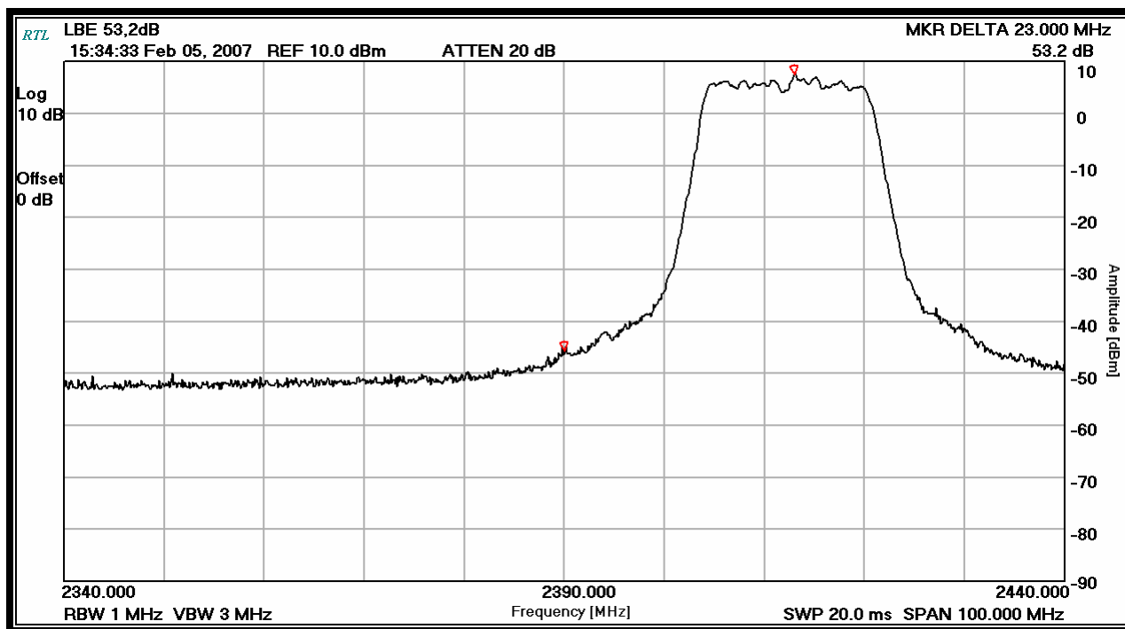
Plot 4-1: Lower Band Edge: Average Measurement Channel 1 (TX Frequency: 2412 MHz)
