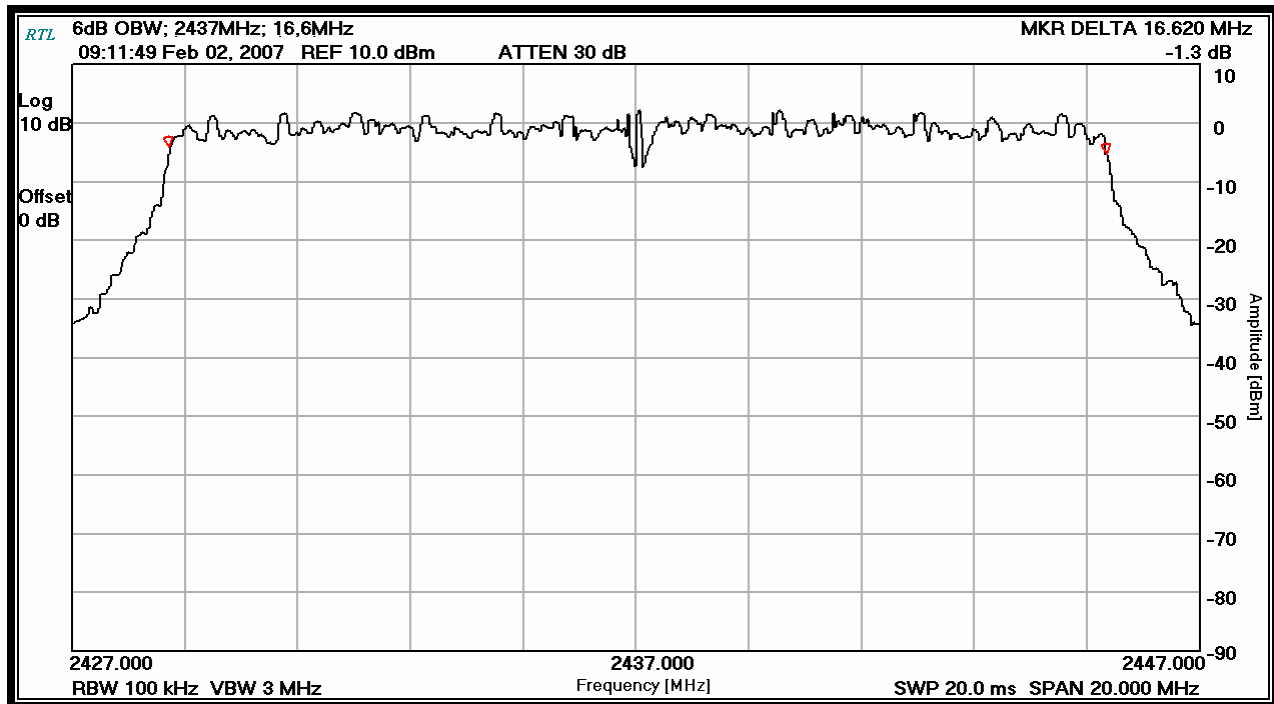
Plot 6-2: 6 dB Bandwidth Channel 6 (TX Frequency: 2437 MHz)
