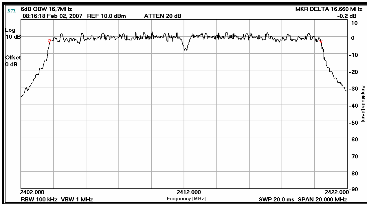
Plot 6-1: 6 dB Bandwidth Channel 1 (TX Frequency: 2412 MHz)
