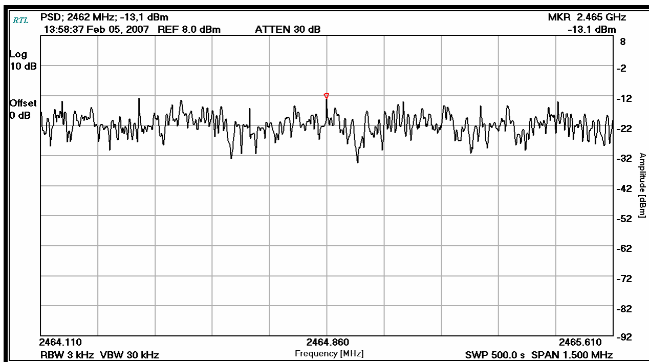
Plot 7-3: Power Spectral Density: Channel 11 (2462 MHz)
