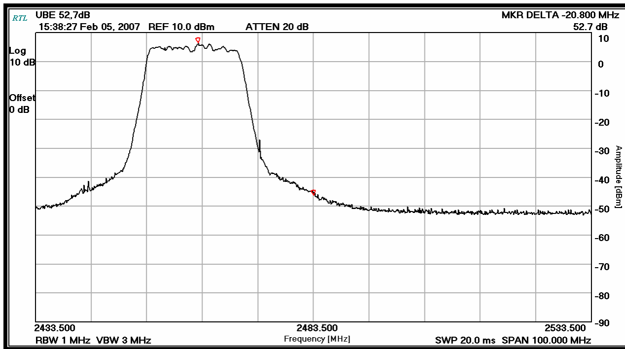
Plot 4-2: Upper Band Edge: Average Measurement Channel 11 (TX Frequency: 2462 MHz)
