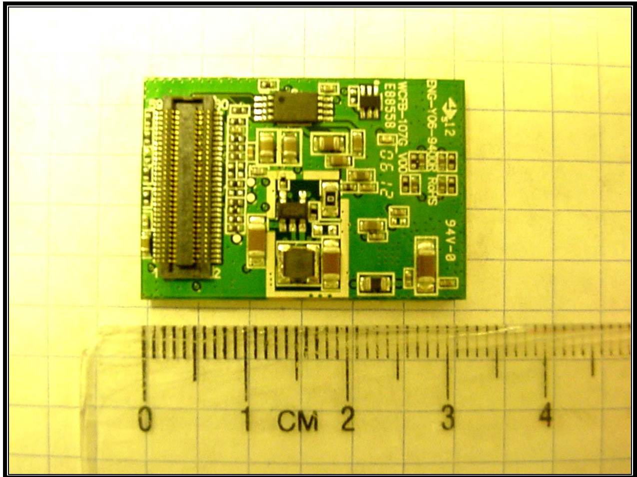
Photograph 17: Radio Bottom View
