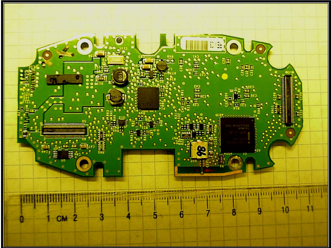
Photograph 14: PCB Back View, Without WLAN Radio
