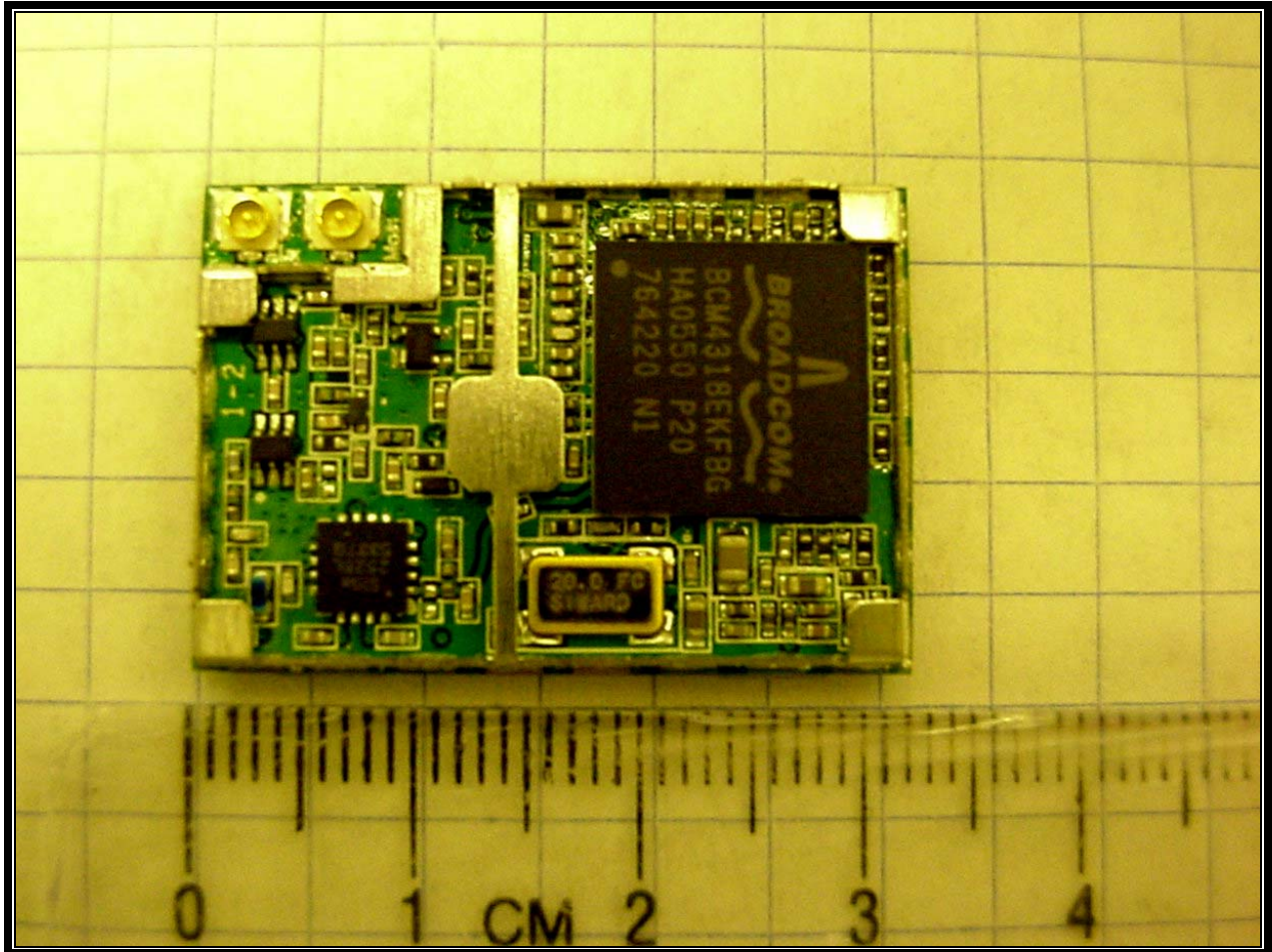
Photograph 16: Radio Top View, Without Shield
