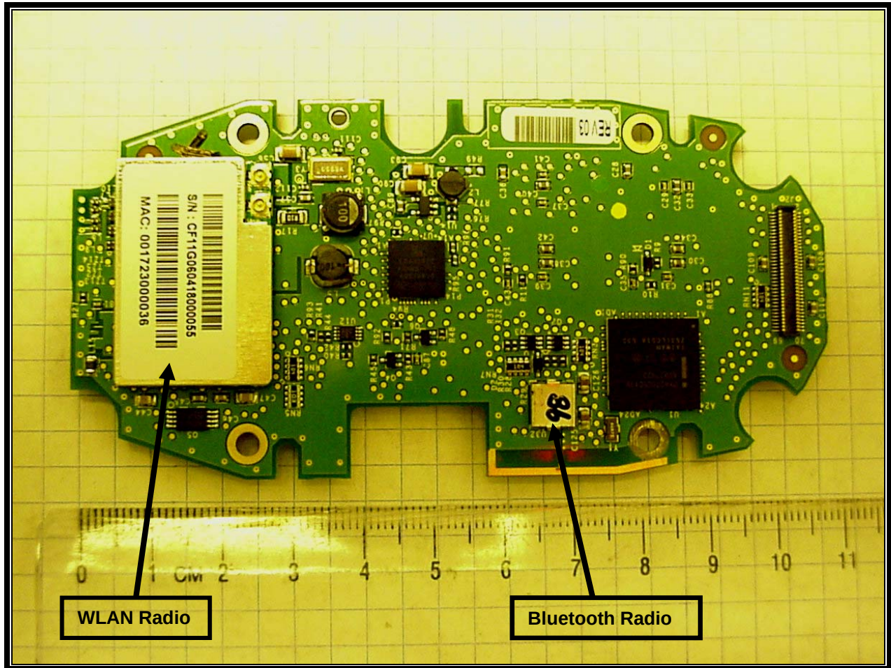
Photograph 13: PCB Back View, With WLAN Radio
