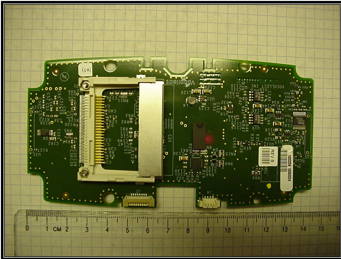
Photograph 12: Top PCB
