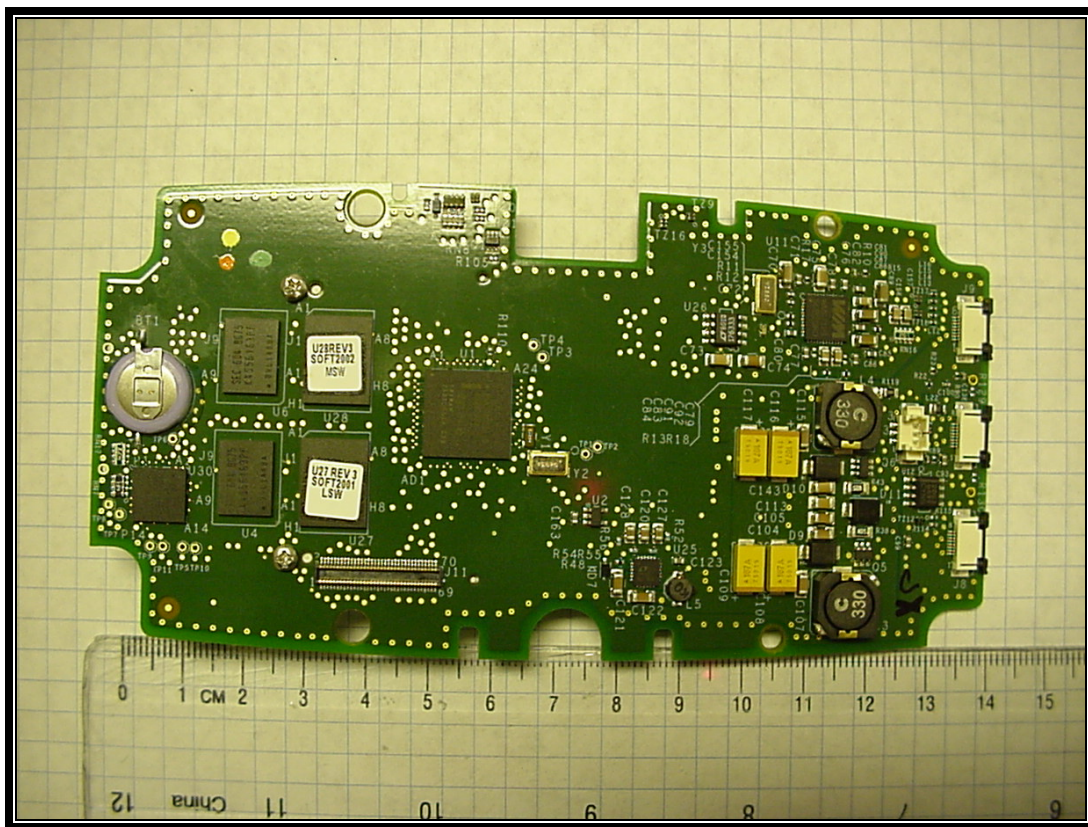
Photograph 13: Bottom PCB
