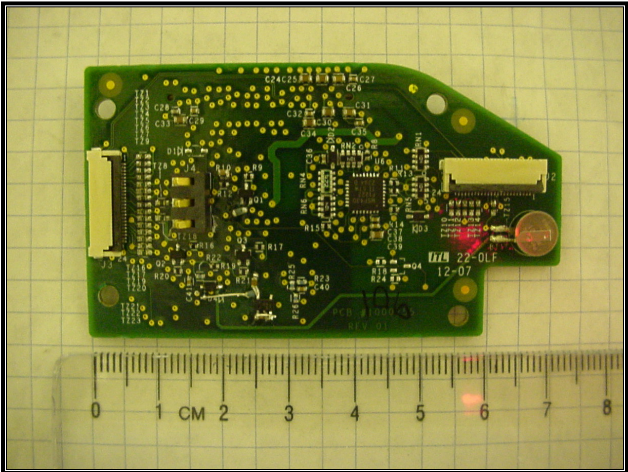
Photograph 11: Bottom PCB Showing Battery Connection
