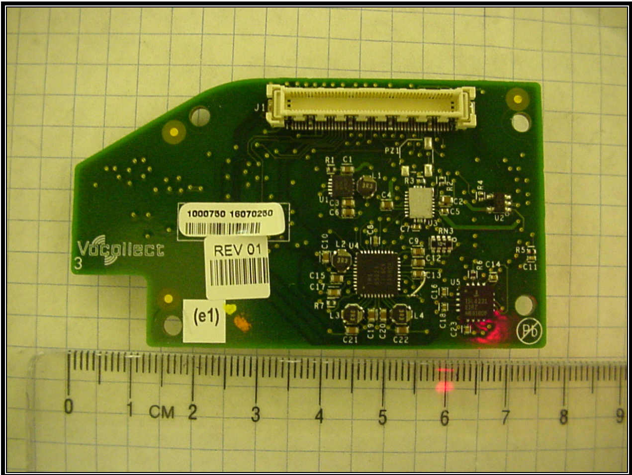
Photograph 12: Top of Bottom PCB
