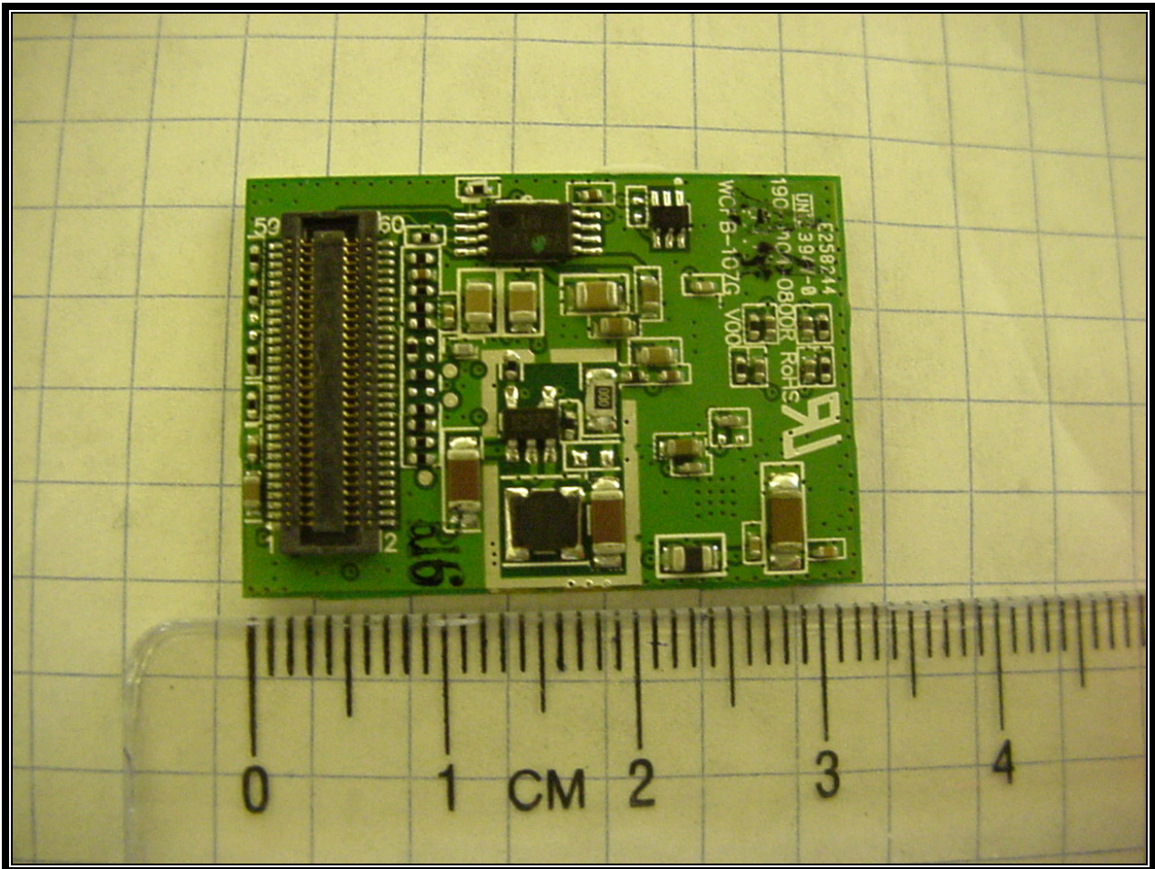
Photograph 20: Bottom of Radio
