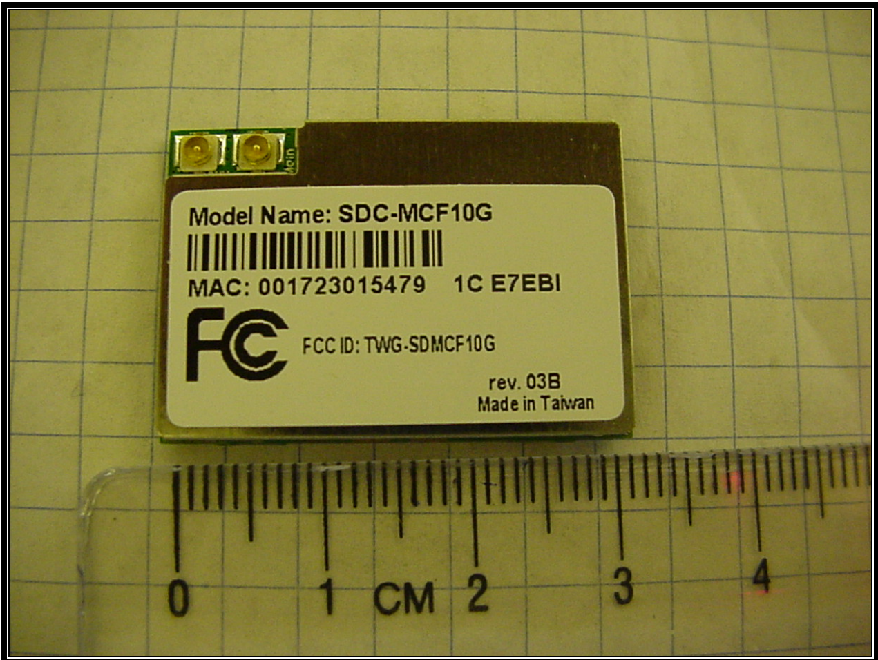
Photograph 18: Top of Radio Card with Shield
