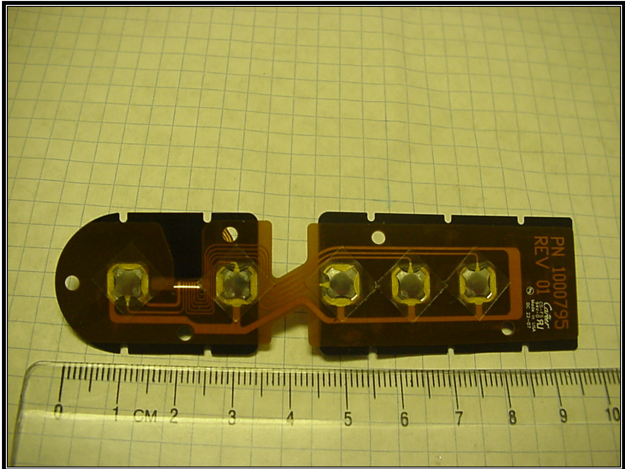
Photograph 17: Side Button PCB
