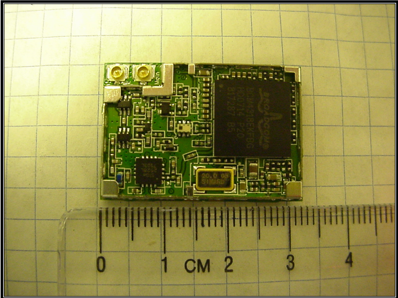
Photograph 19: Top of Radio with Shield Removed
