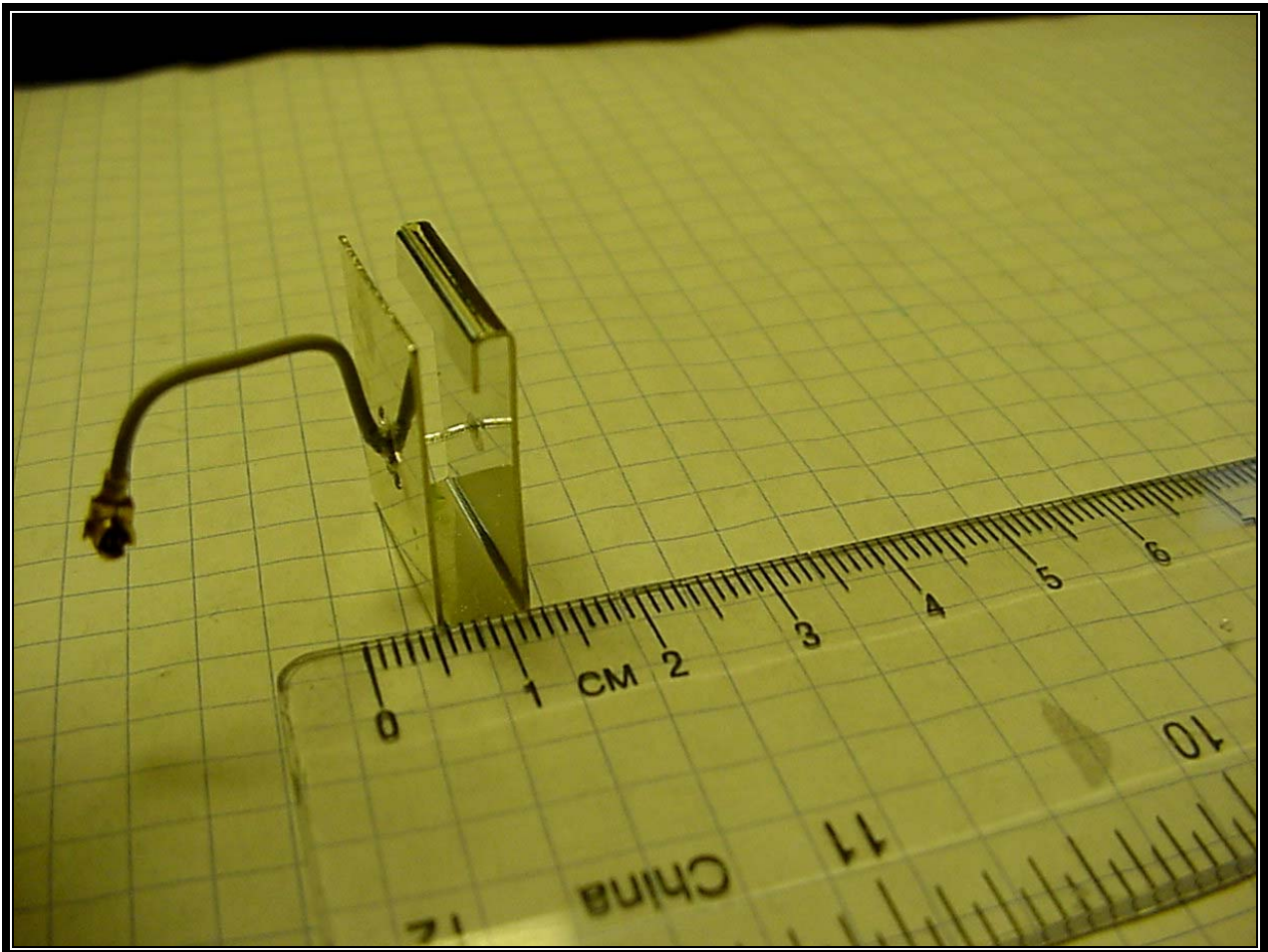
Photograph 16: Antenna
