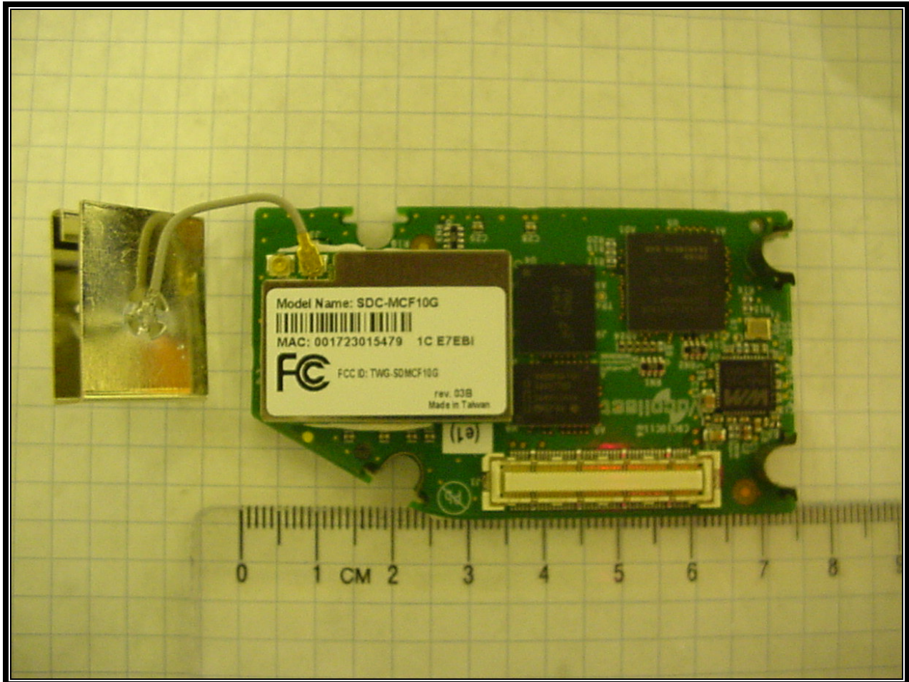
Photograph 13: Bottom of Top PCB Showing Radio with Shield and Antenna Connected
