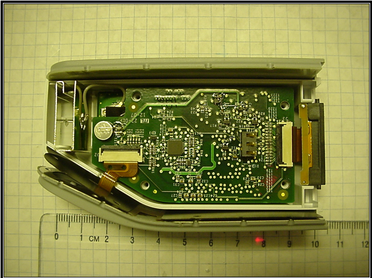
Photograph 10: Bottom PCB in Case
