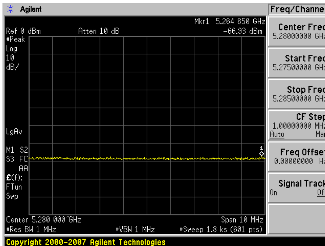
Figure 5-10 Non-occupancy Period - Monitoring live real time spectrum - Elapse time 30 minutes
