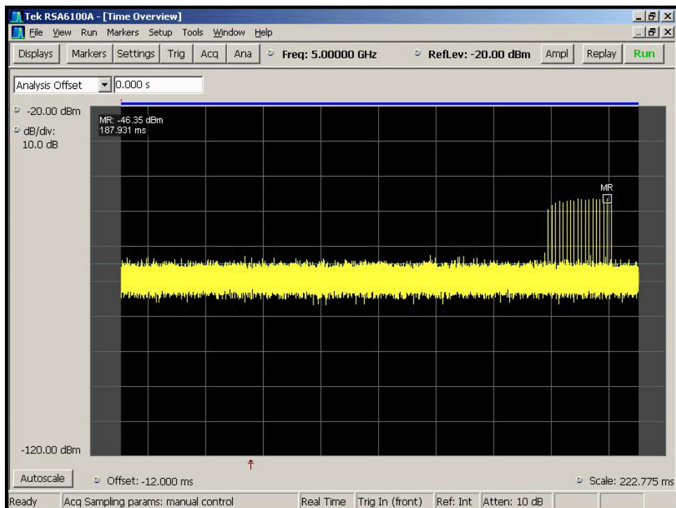
Figure 5-1. Sample Type 1 Radar Pulse
