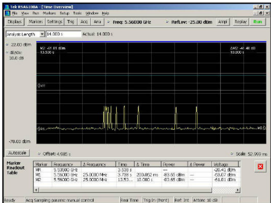
Figure 6-6. Aggregate Time of Pulse Grouping approx. 1 second from radar pulse
