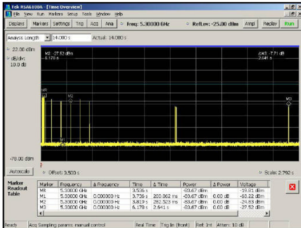
Figure 5-6. Entire Channel Closing Transmission Time, Aggregate Time After 200ms
