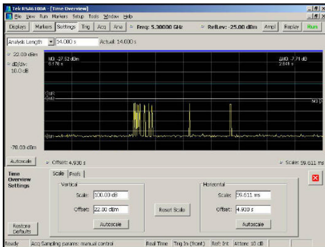
Figure 5-7. Aggregate Time of Pulse Grouping approx. 1 second from radar pulse
