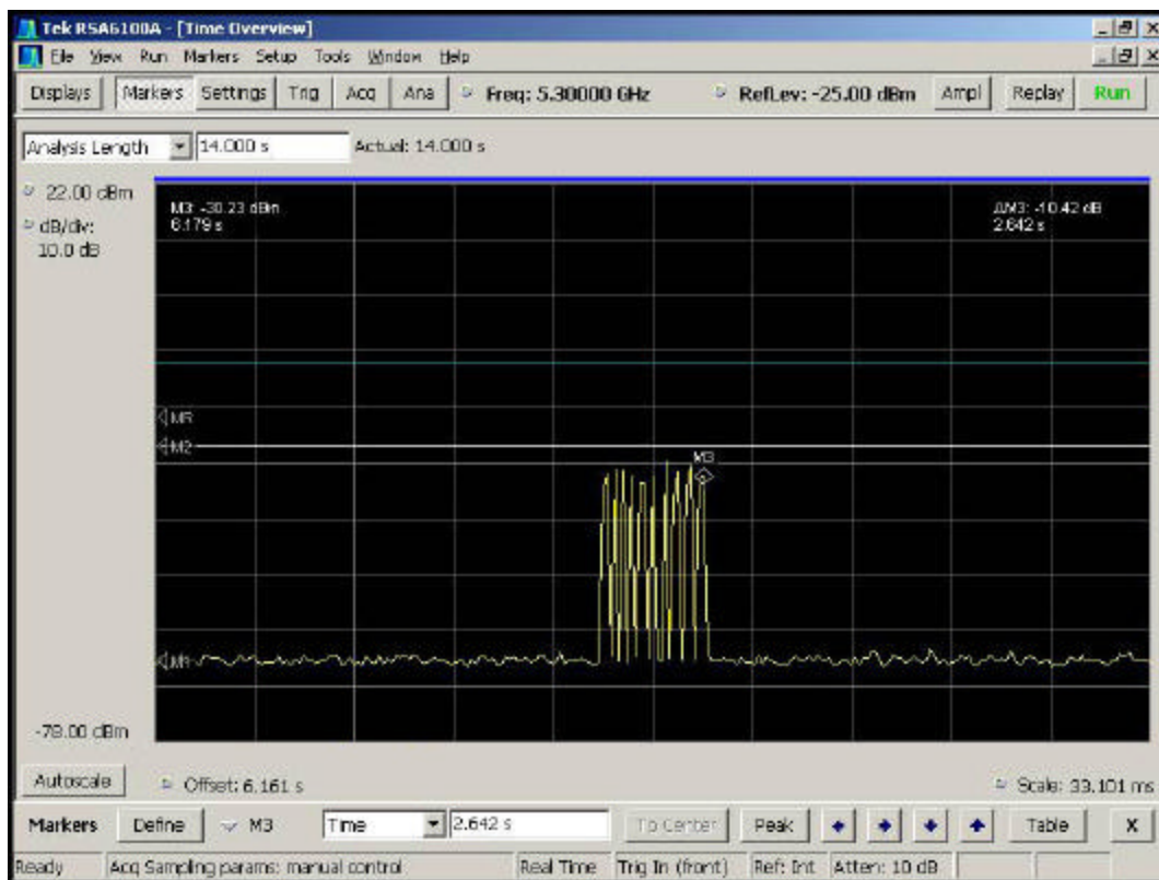
Figure 5-8. Aggregate Time of last Pulse Grouping 2.6 seconds from radar pulse
