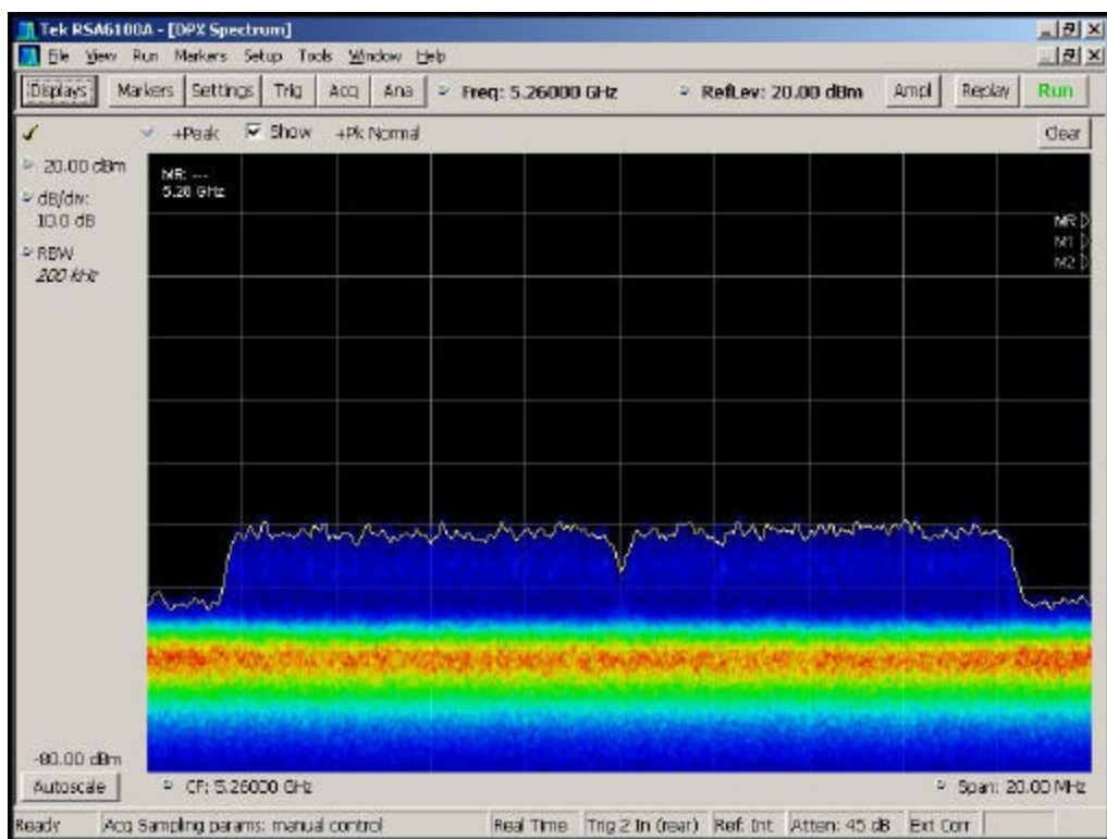
Figure 5-4. Real-Time Spectrum Display, WLAN Traffic
