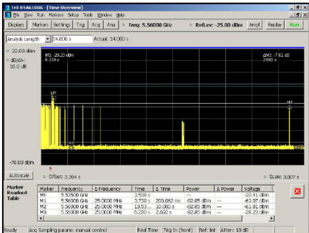
Figure 6-5. Entire Channel Closing Transmission Time, Aggregate Time After 200ms
