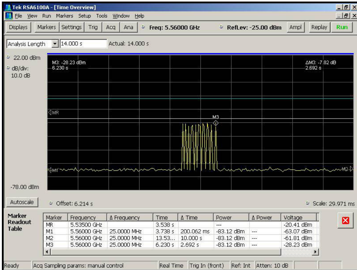
Figure 6-7. Aggregate Time of Pulse Grouping approx. 2.6 second from radar pulse
