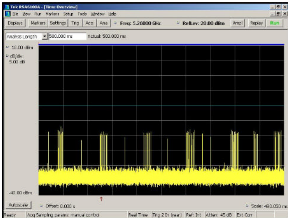
Figure 5-2. Time Display WLAN Channel Traffic
