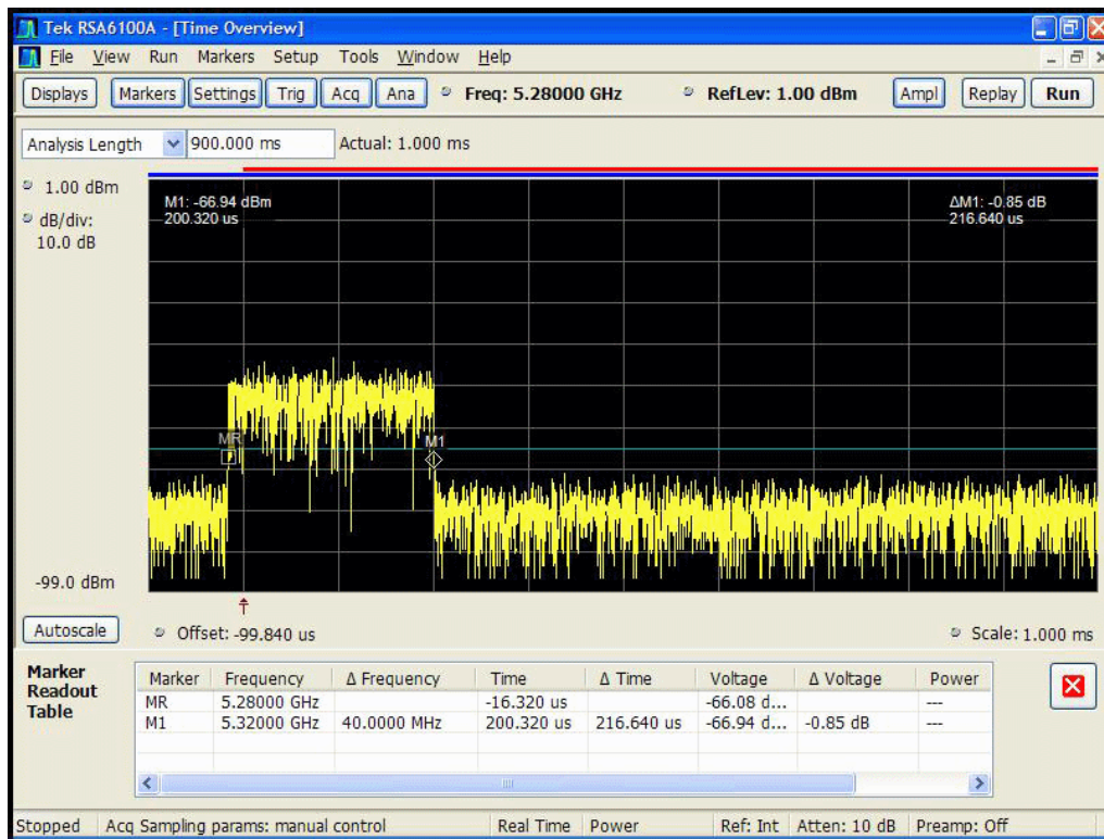
Figure 5-9. Pulse Width After 200ms
