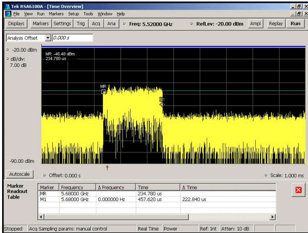
Figure 6-8. Pulse Width After 200ms
