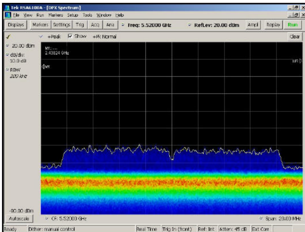
Figure 6-3. Real-Time Spectrum Display, WLAN Traffic
